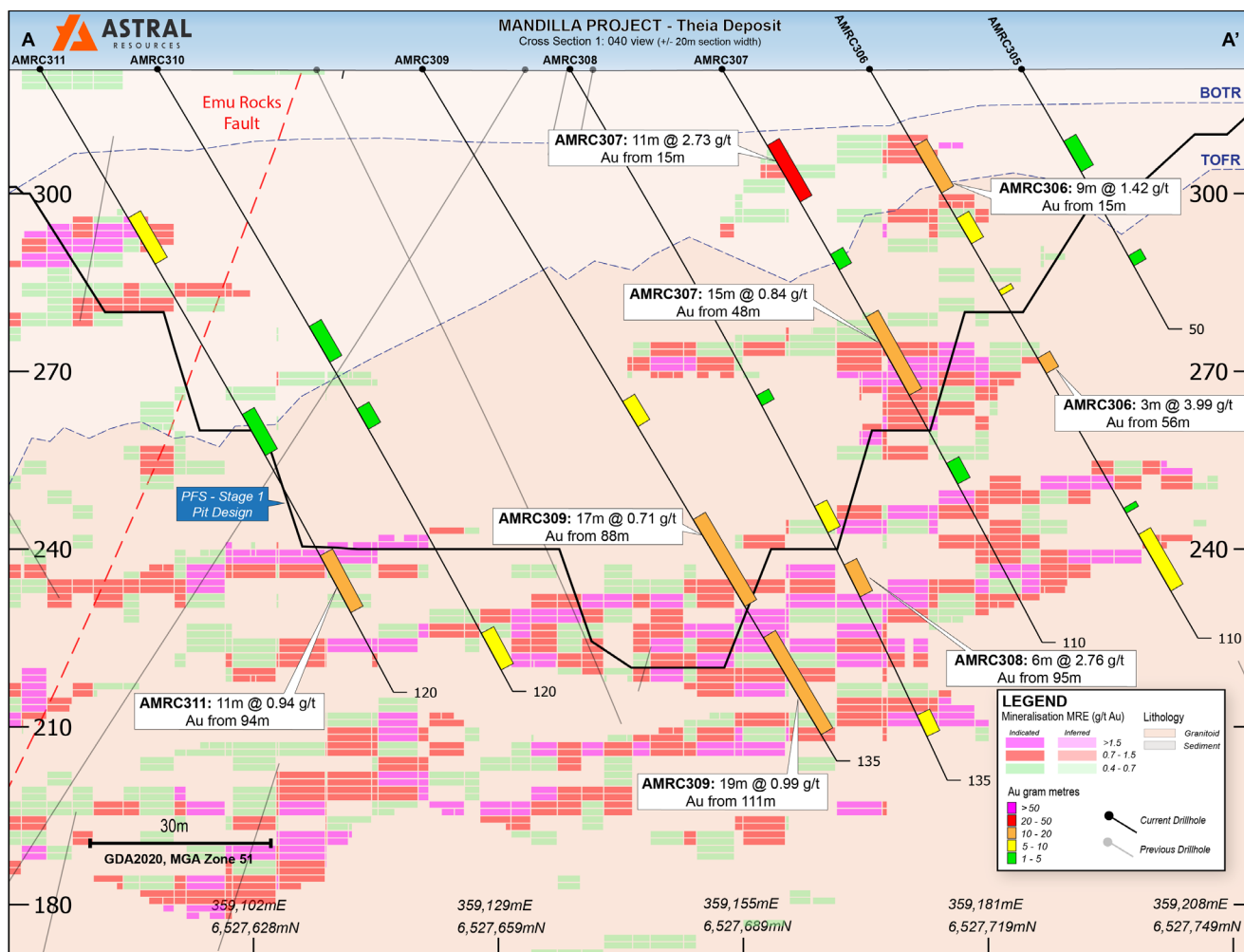
Figure 3 – Cross-section A-A' view of the Theia Deposit showing the drill trace and assay results for the current in-fill RC drilling (please note - previous drillholes are not drawn with reported assay intervals).
