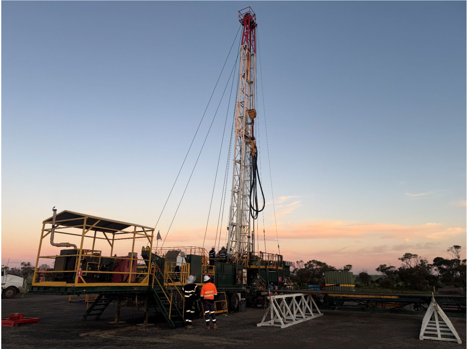
Figure 1: SWS Rig 04 on site at Ramsay 1
