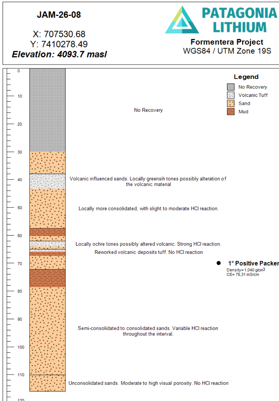
Figure 1. Figure 1. JAM 26-08 Cilon lithology column showing brine assay with 1.04gm/cm 3 with porous sands, but void of carbonates
