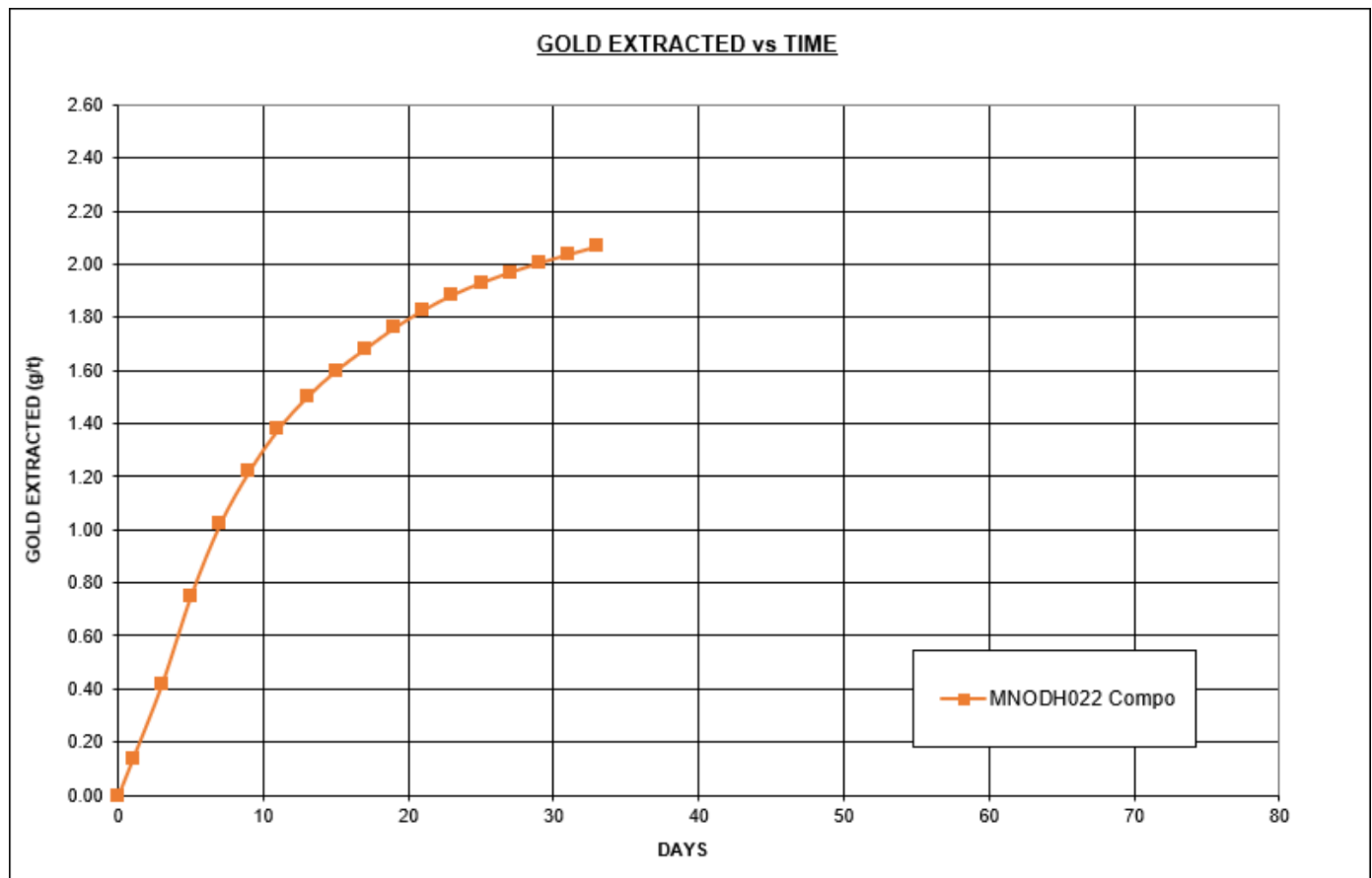
Figure 3: MNODH 022 Gold recovered in solution (g/t Au) vs time, in days – Column test still underway
