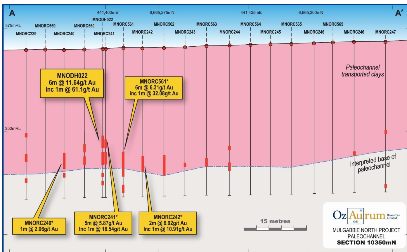
Figure 5: James cross section 10350N
