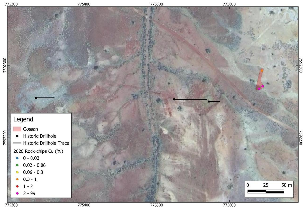
Figure 5: Plan view of the historic drillholes trace with gossan location.
