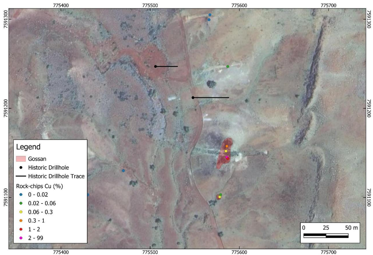
Figure 6: Plan view of the historic drillholes trace with gossan location.
