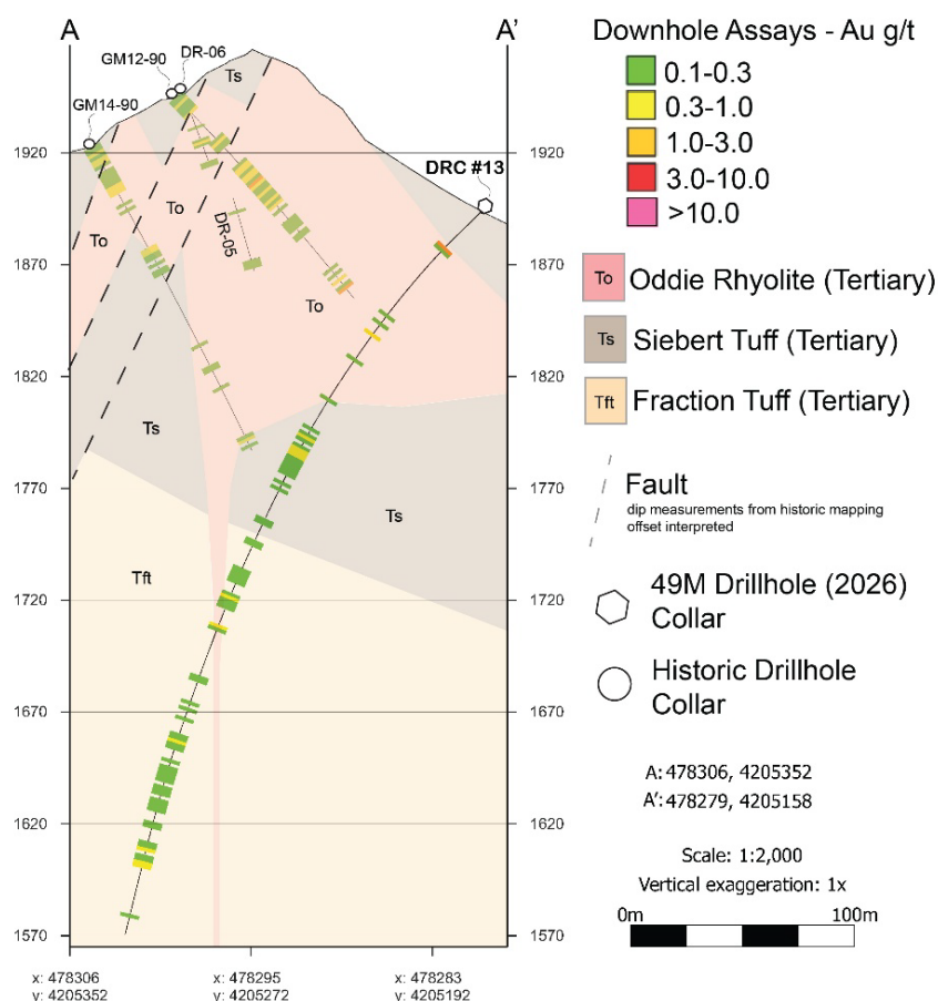
Figure 5: Cross Section of DRC#13
