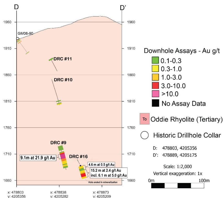
Figure 2: Long Section of the Holes DRC#9 and DRC#16
