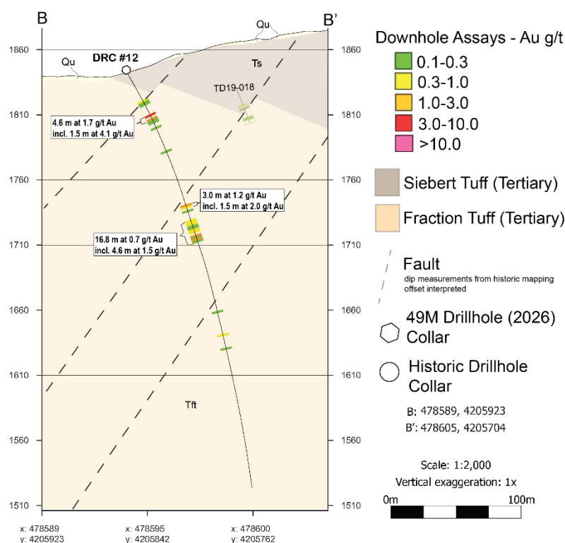
Figure 4: Cross Section of DRC#12
