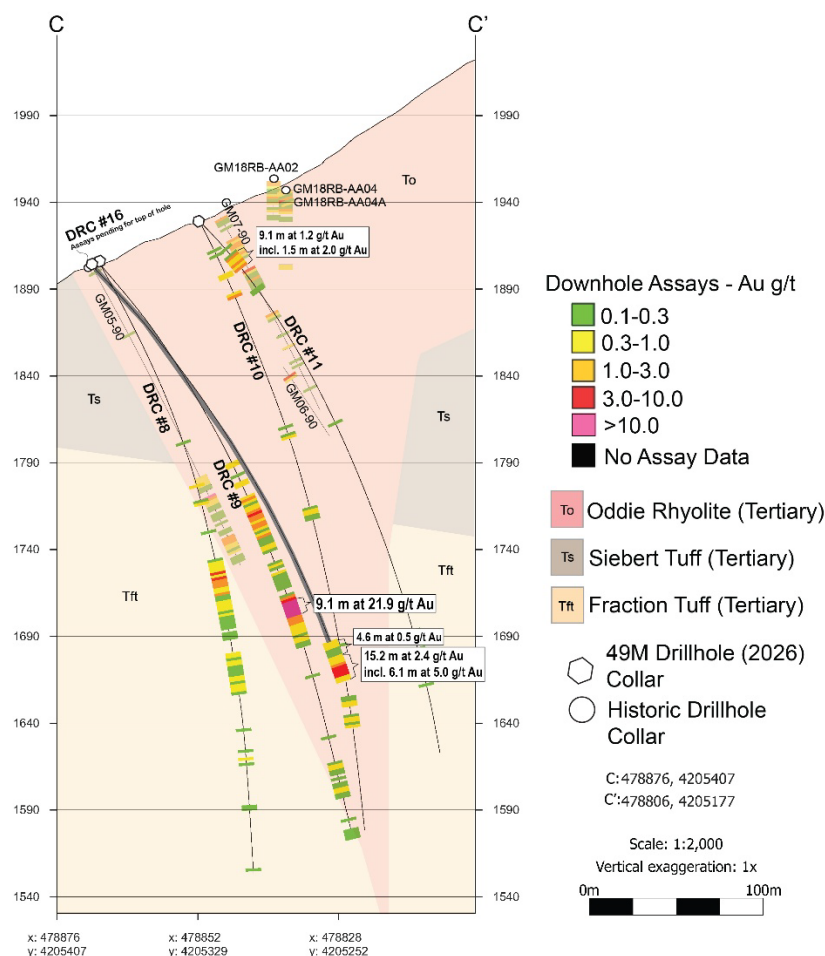
Figure 3: Cross Section of the Adit Zone
