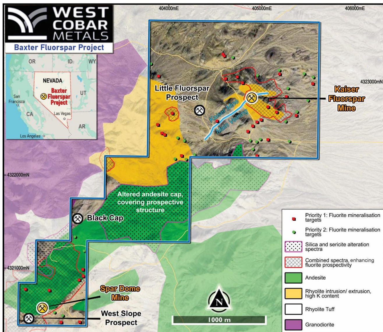
Figure 2: Interpreted geology, historical fluorite workings and areas of selected Sentinel-2 spectra indicating sericite, silica, clay alteration and iron oxides. Based on publicly available Sentinel-2 spectra and aerial radiometric survey. 4 Priority rankings are based on spectral criteria only and require field validation.
