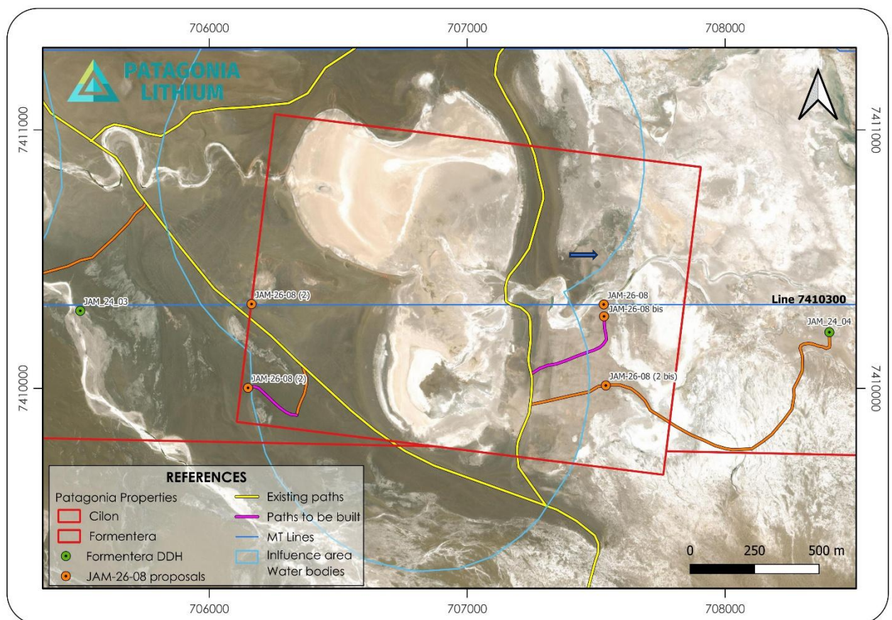
Figure 2. Well eight positioned against MT geophysics. We could not drill directly into the pink (low resistivity) area due to unstable ground filled with brines (ASX:PL3 "MT Geophysics Defines Significant Prospective Drill Targets" on 15 June 2023).
