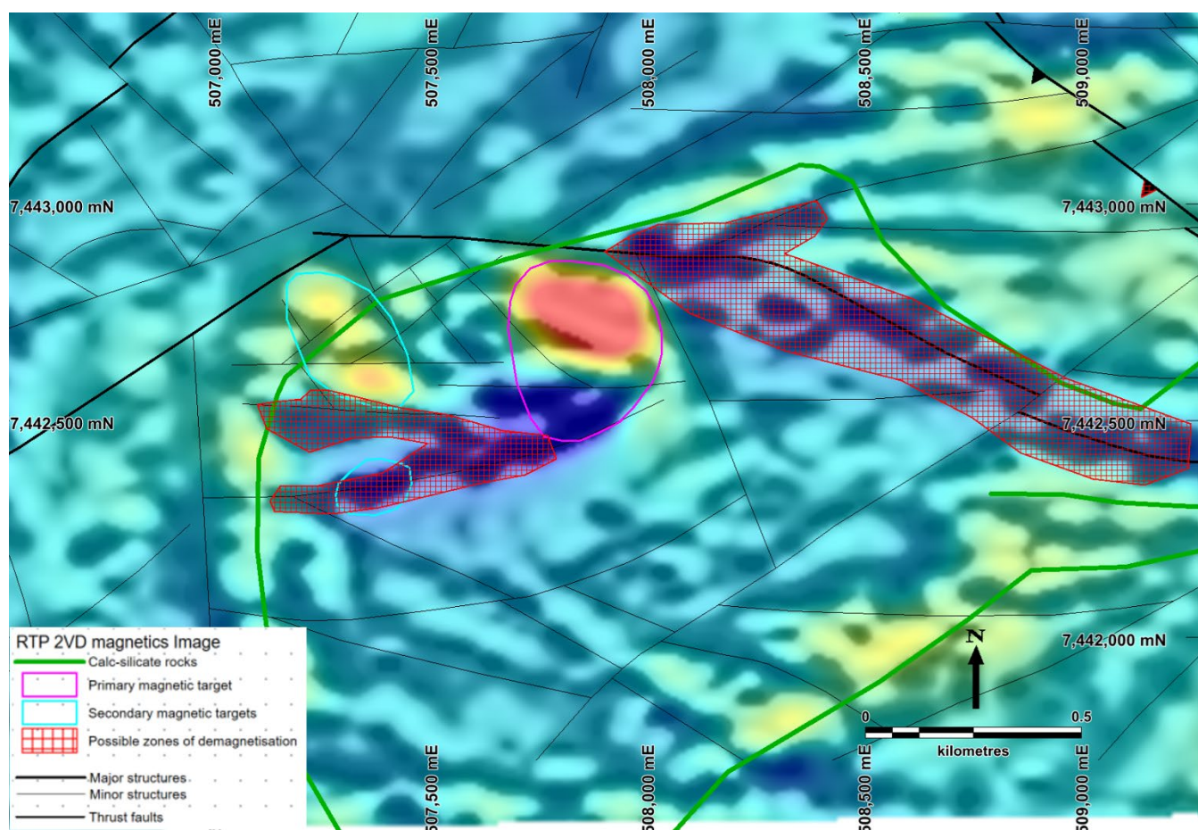
Figure 3: RTP magnetics highlighting the primary Kings Cross magnetic anomaly
