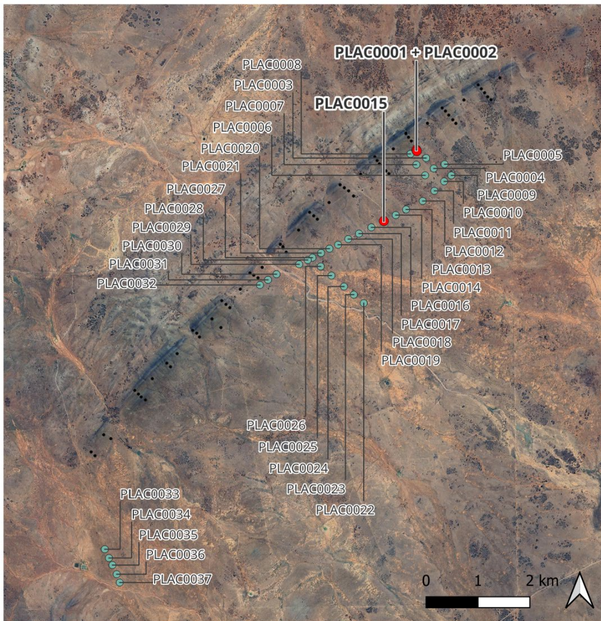
Figure 1. Ironback Hill Drill collar location plan.
