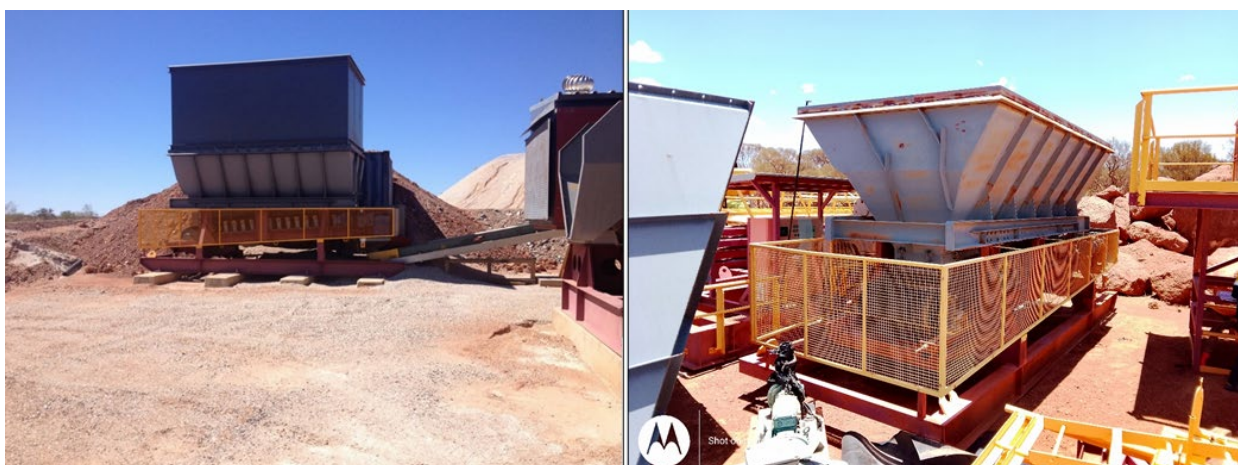
Figure 3: ROM Bin Components
