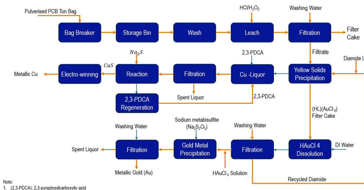
Figure 1 – GCDE Process Block Diagram
