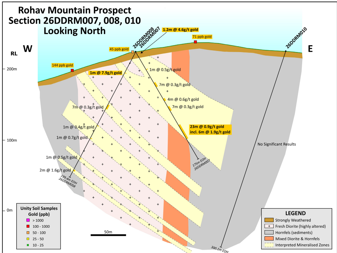
Figure 3: Cross Section of geology revealed by drilling at Rohav Mountain Prospect with significant gold mineralised intervals shown. This relatively shallow-dipping mineralisation lies within intensely phyllic altered diorite that has also been heavily stockwork veined eastern contact of the diorite intrusion.
