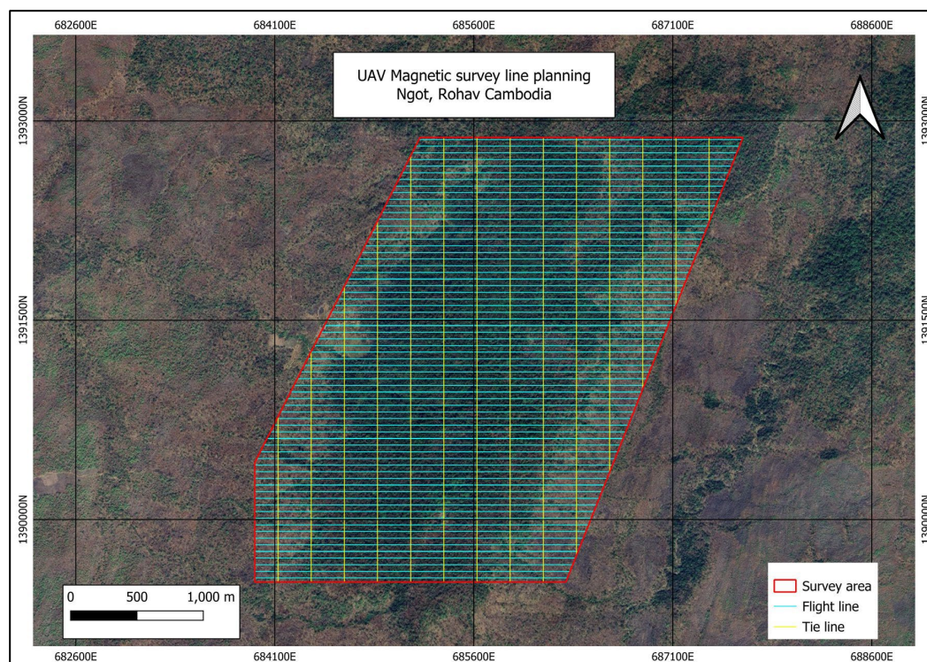
Figure 4 : Proposed UAV Magnetics and LiDAR coverage area at Rohav Mountain.
