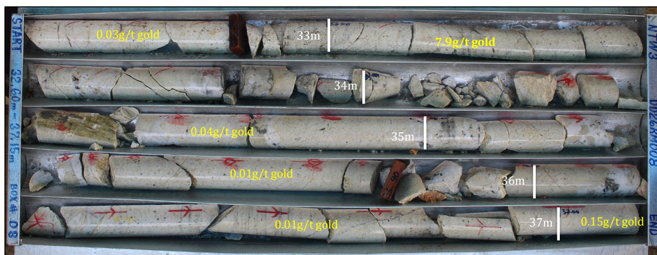
Figure 2: Photograph of diamond drill hole 26DDRM008 from 32.60 m to 37.15 m (downhole) at Rohav Mountain, showing the highly altered diorite host rock, the multi-generational stock work quartz veins and the reported intersection of 1 m @ 7.9 g/t gold from 33 – 34 m . All assay and interpretive information was reported on previously, ASX News Release 20th April 2026. Intensely mineralised zones of stockwork veins and strong alteration occur throughout the diorite, however gold is closely associated with a later generation of vuggy quartz veins with strong poly-metallic sulphides (pyrite – arsenopyrite – sphalerite and lesser galena).
