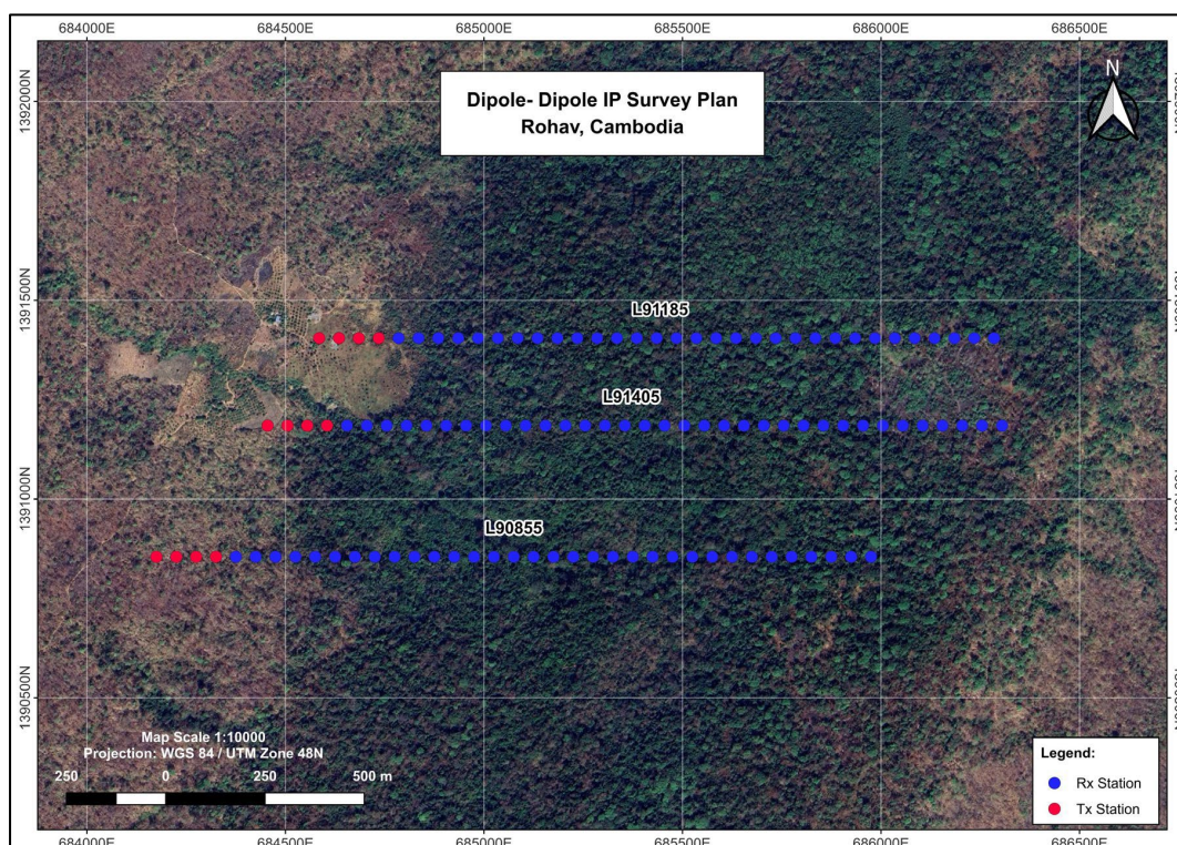
Figure 5: Proposed new Rohav Mountain DDIP survey lines.
