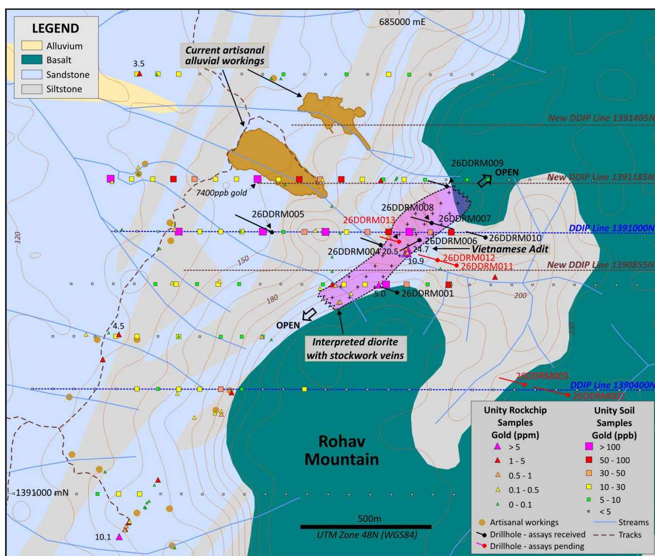
Figure 1: Gold in soil anomalies, rock chip sample gold results, drill holes locations at the Rohav Mountain Prospect on interpreted geology.
