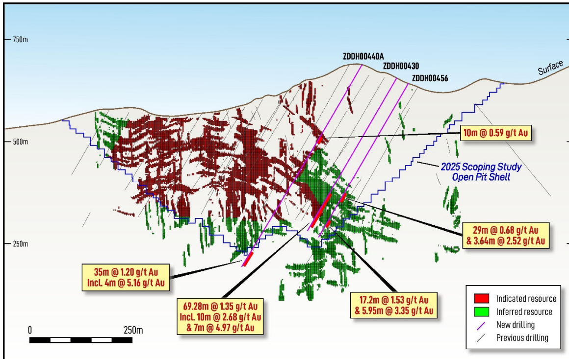
Figure 2: El Zorro Gold Project –Drilling section A-A'. Showing holes ZDDH0440A, ZDDH0430 and ZDDH0456 and resource classification of current MRE block model. Holes displayed are projected onto section +/-20m. Looking northwest. Datum PSAD56 19S. Refer ASX announcement 30 April 2026 for results from ZDDH0430.
