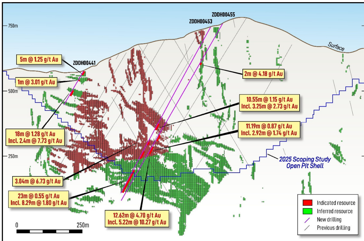
Figure 3: El Zorro Gold Project –Drilling section B-B'. Showing holes ZDDH0441, ZDDH0453 and ZDDH0455 and resource classification of current MRE block model. Holes displayed are projected onto section +/-20m. Looking northwest. Datum PSAD56 19S.
