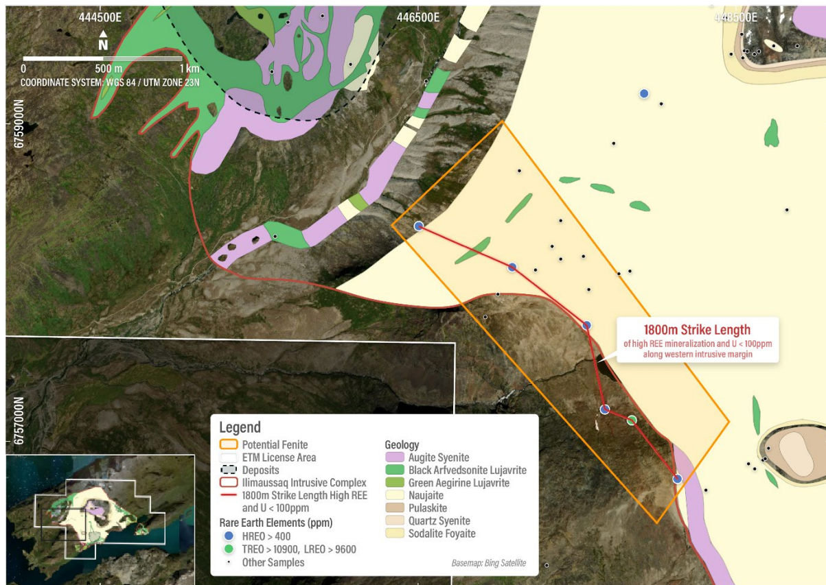
Figure 4. A) Rock samples that are enriched in TREO, LREO, and/or HREO (greater than the average Kvanefeld deposit grade) and also less than 100 ppm uranium. B) 1,800 m trend of mineralized HREO samples, with uranium less than 100 ppm (see Table2).
