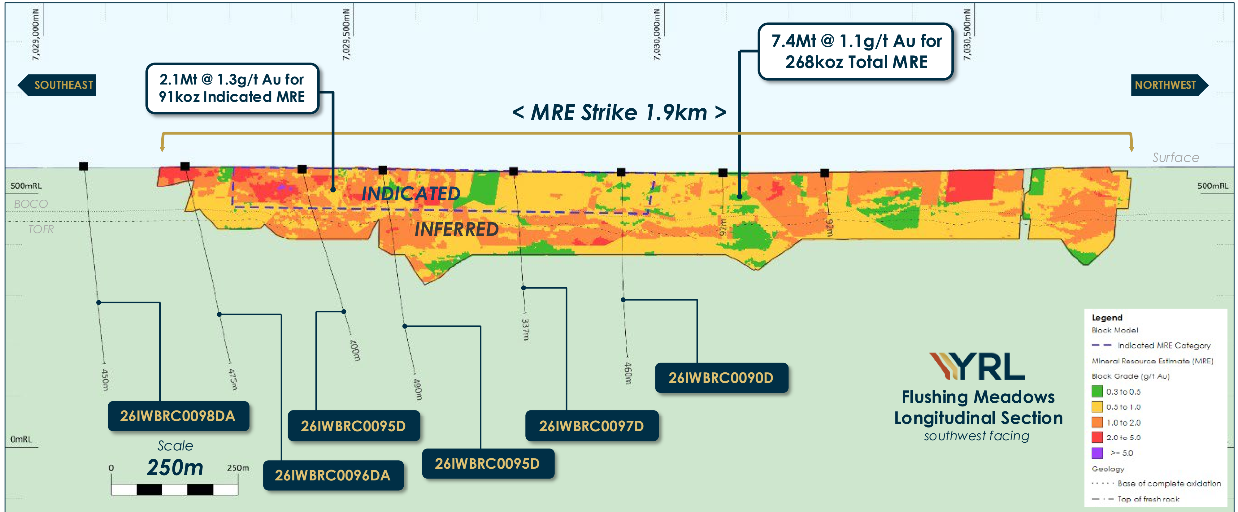
Flushing Meadows longitudinal section showing MRE block model and recent diamond drilling from ASX Release 9 June 2026.
