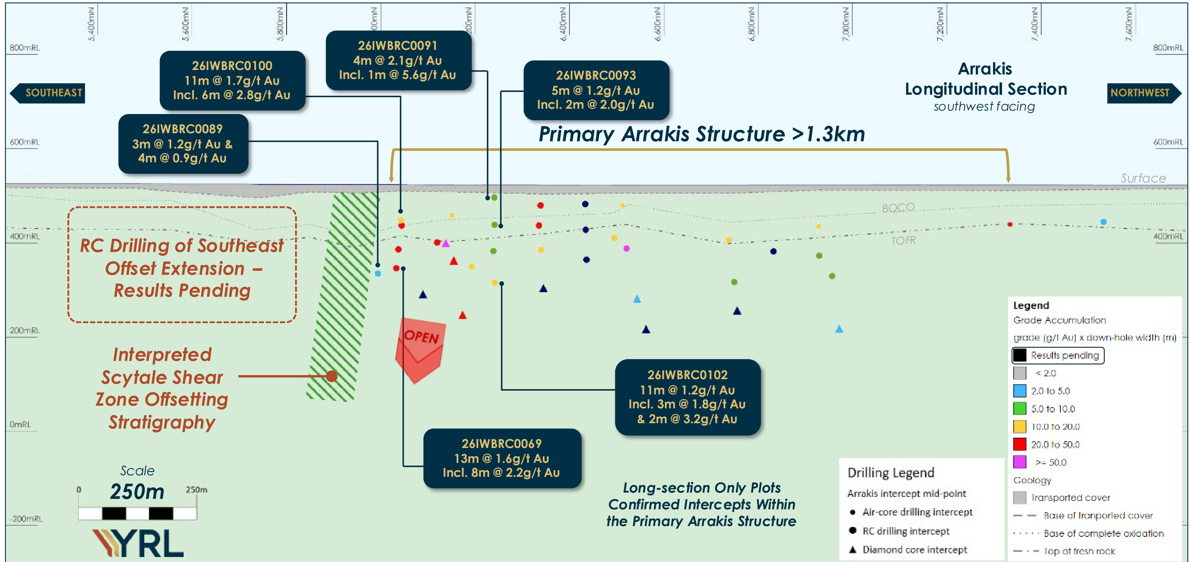
Arrakis longitudinal section showing all intercepts within the main mineralised structure from ASX Release 9 June 2026.
