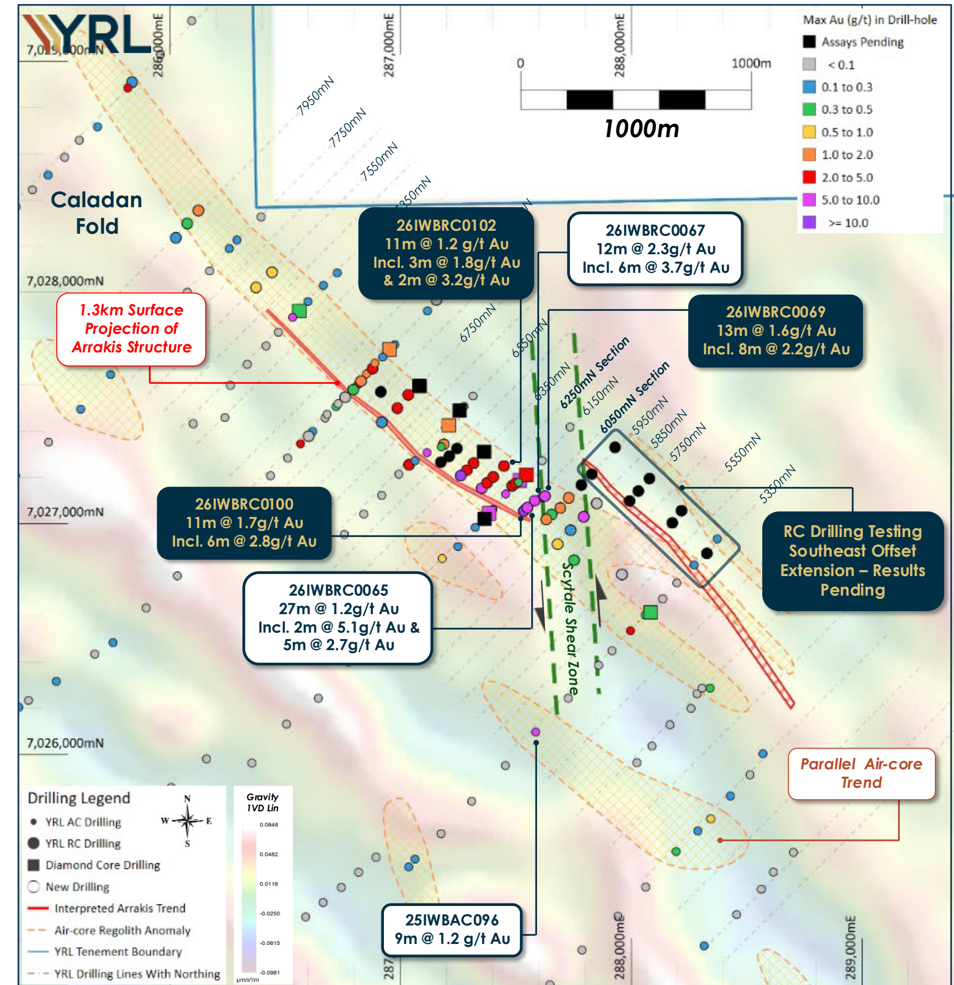
Arrakis collar plan, see ASX release 9 th June 2026
