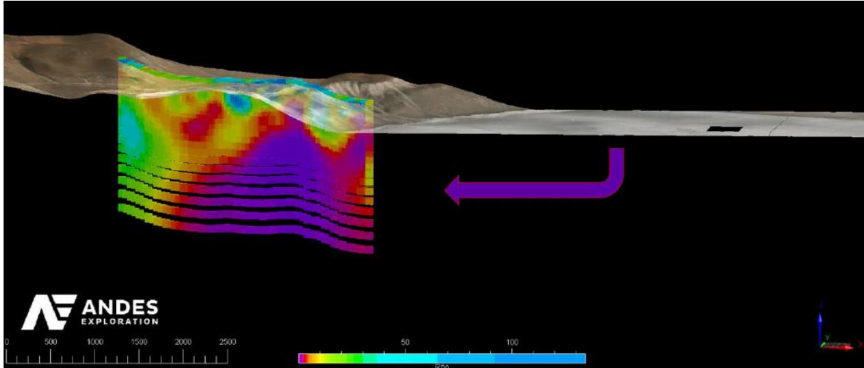
Figure 3 – CSAMT Cross Section L1500 Showing a Deep, Continuous Conductive Zone Interpreted as a Priority Brine Target Adjacent to the Newly Acquired Project Areas.
