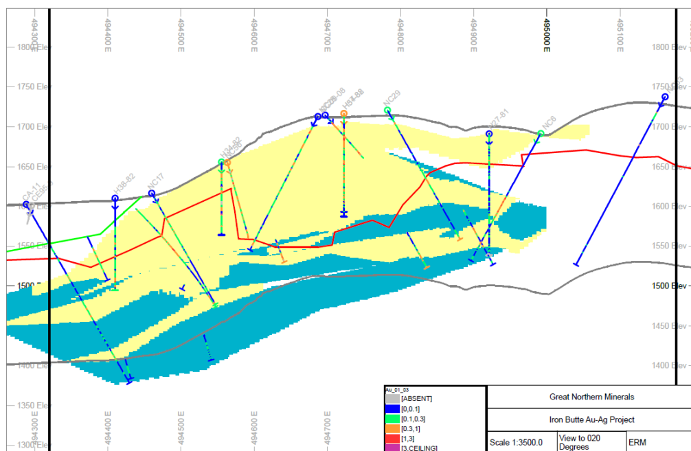
Figure 6: Cross section view to 020°, showing Inferred resource (yellow – AUZONE, blue – AGZONE); topographic surface, base of alluvium (green), base of oxidation (red), drill holes; base of resource reporting surface (grey); and claim (black).
