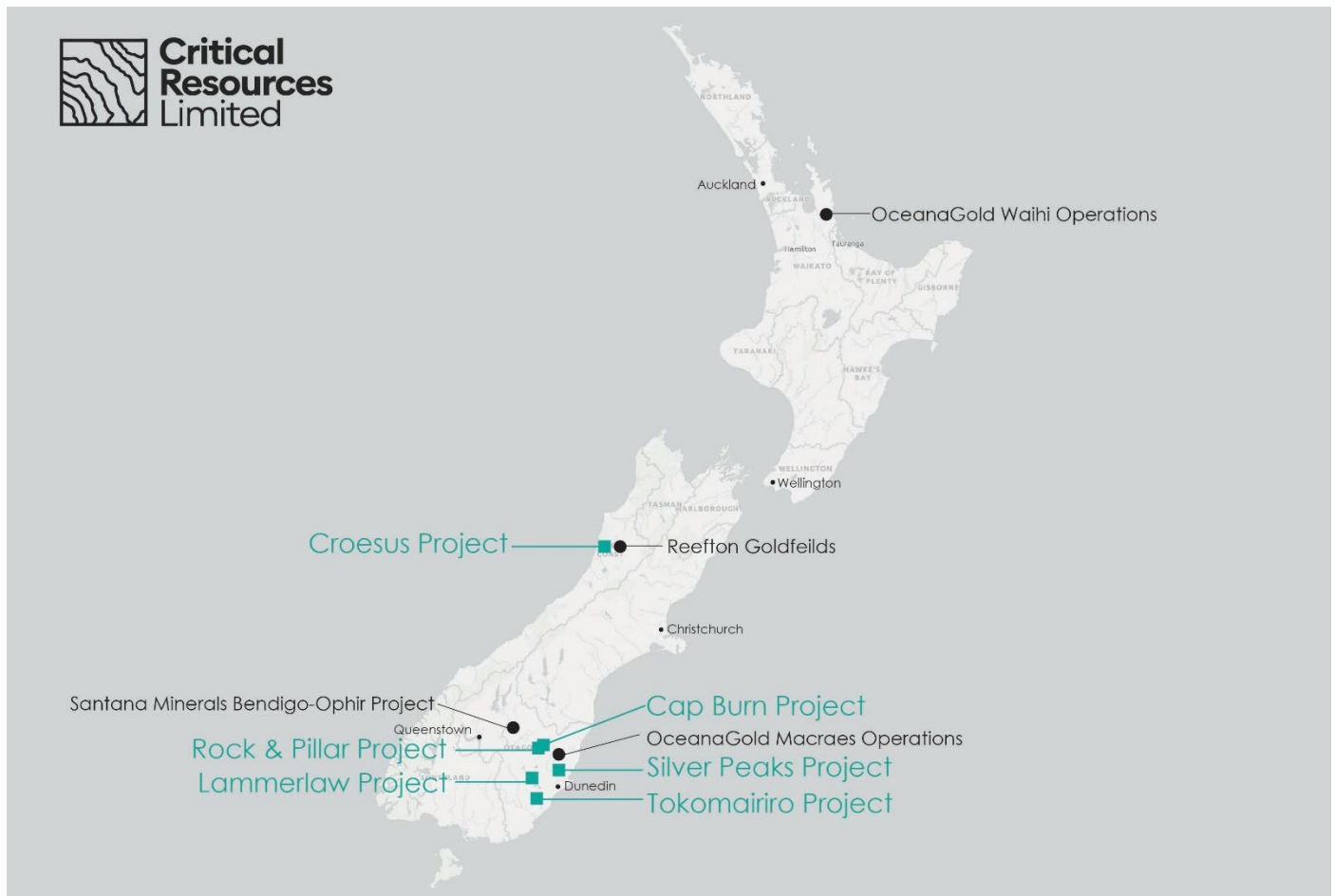
Figure 4 - Location of Critical Resources' New Zealand gold projects with Major Gold Projects.
