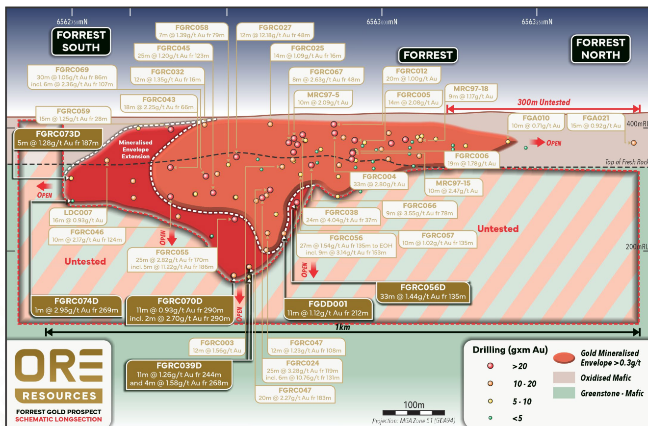
Figure 3: Forrest Schematic – Long Section
