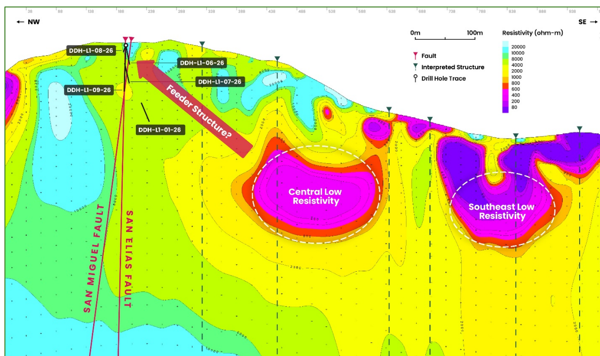
Figure 1: Lirios 1 CSAMT survey, Line 2: 2D inversion model resistivity section with drillholes on \pm 15 m on section showing the two potential sulphide related resistivity lows and feeder network.
