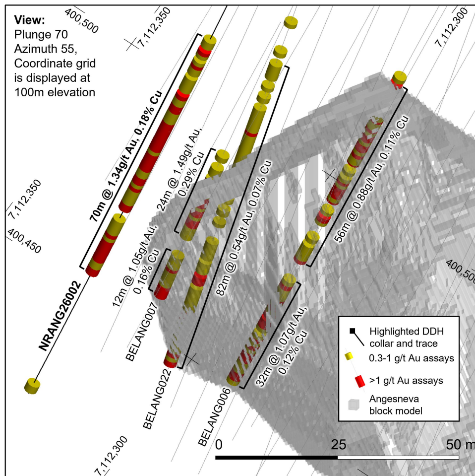
Figure 4: 3D image of the block model (grey shell) from the northern end of the Angeneva resource showing NRANG26002 and the historical holes nearby. The gold mineralisation intersected is shown along the drill traces. See Appendix 1 and Appendix 2 for the drill hole details. Coordinates presented in ETRS-TM35FIN system (EPSG:3067).
