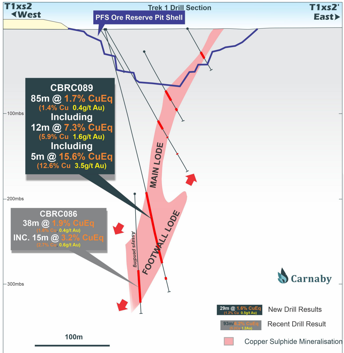
Figure 5. Trek 1 Cross Section showing new Footwall Lode drill results.
