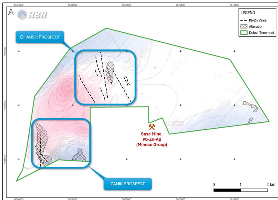
Figure 4: Dolovi tenement, airborne magnetic survey (ASX Ann 31.03.2026)
