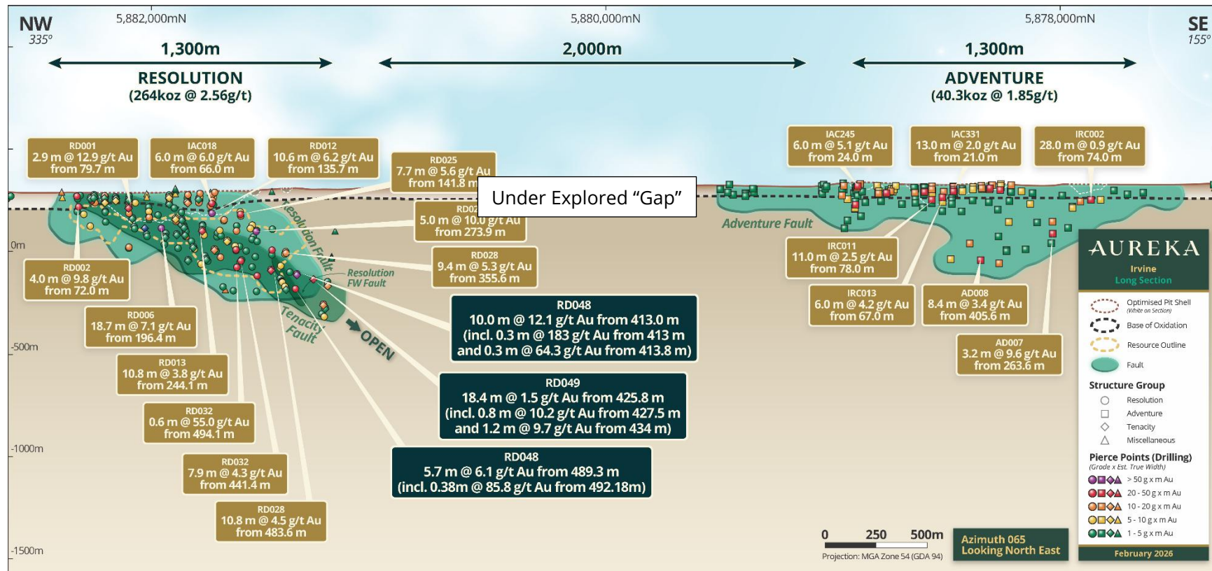
Figure 4: Targeting the gap between Resolution and Adventure lodes: Irvine Long Section with current drilling and intercepts outside current JORC Resource 10 and underexplored 2,00m "Gap" between Resolution and Adventure where the high resolution magnetic survey data has enhanced drill targeting
