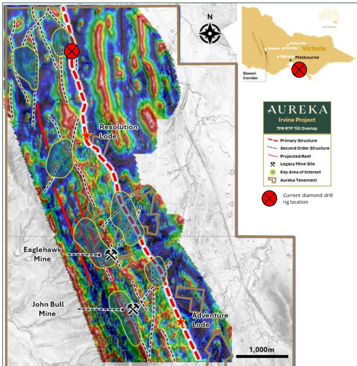
Figure 2: Drone acquired TMI magnetics, reduced to the pole (RTP) - tilt derivative overlay on topography. The Resolution lode and Adventure lode are marked (red star) and comprise the current lodes that make up the 304koz inferred JORC Resource at the Irvine Gold Project. The red circle with cross indicates current location of diamond drilling underway.
