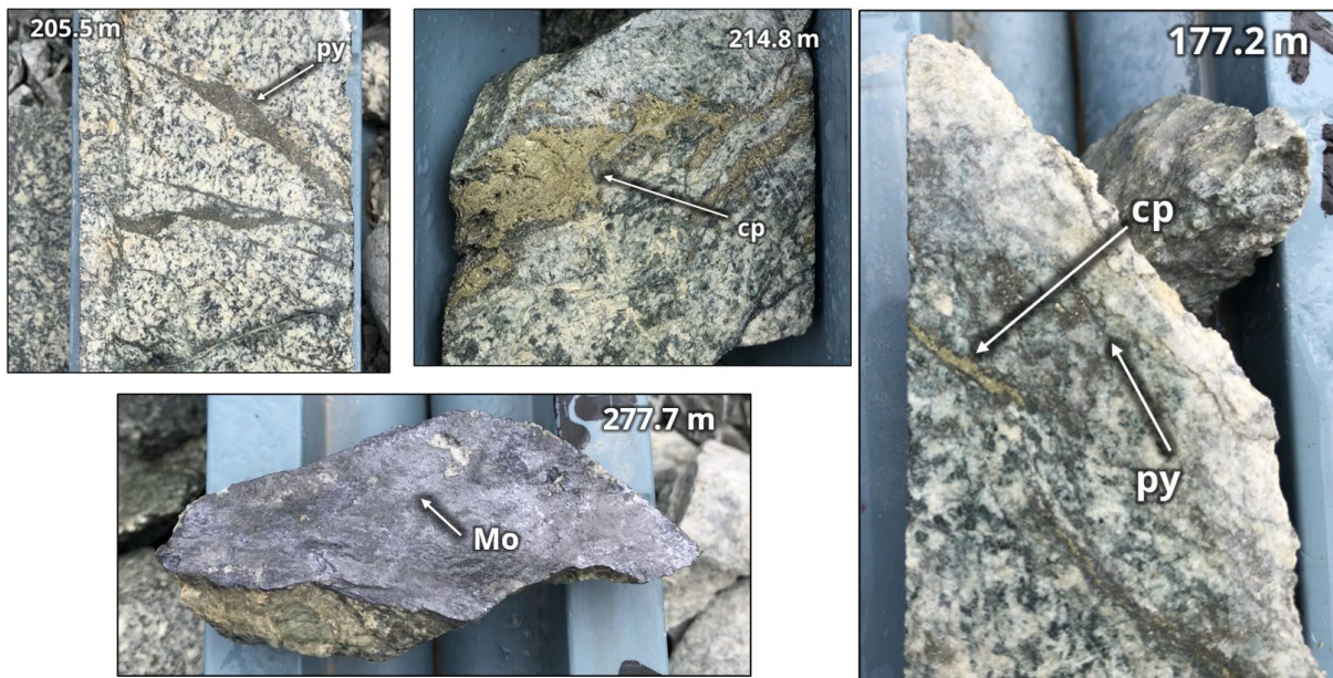
Figure 10: Burringa drill core, photos of mineralisation in quartz-chlorite altered diorite, chalcopyrite (cp), pyrite (py), molybdenite (Mo) JN0025.
