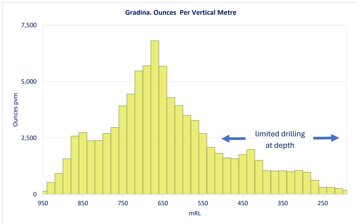
Figure 9. Gradina Inferred Resources Au ounces per vertical metre.
