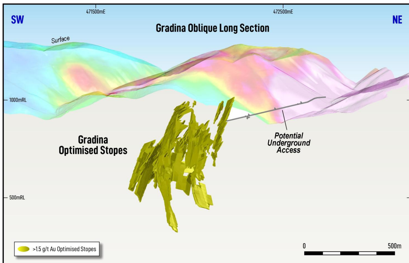
Figure 8. Gradina oblique view, looking northwest, showing optimised > 1.5 g/t Au stopes with conceptual adit access and gold-arsenic soil geochemical anomalism draped over topography.
