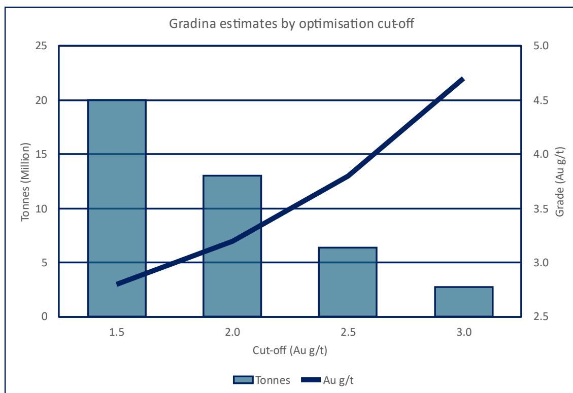
Figure 2. Gradina Long Hole Open Stopping Grade and Tonnage.
