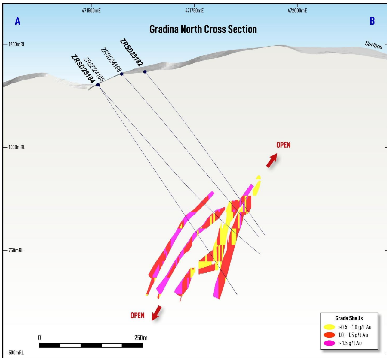
Figure 4. Gradina cross-section along A – B, looking north, showing drill traces and >0.5g/t Au model blocks.
