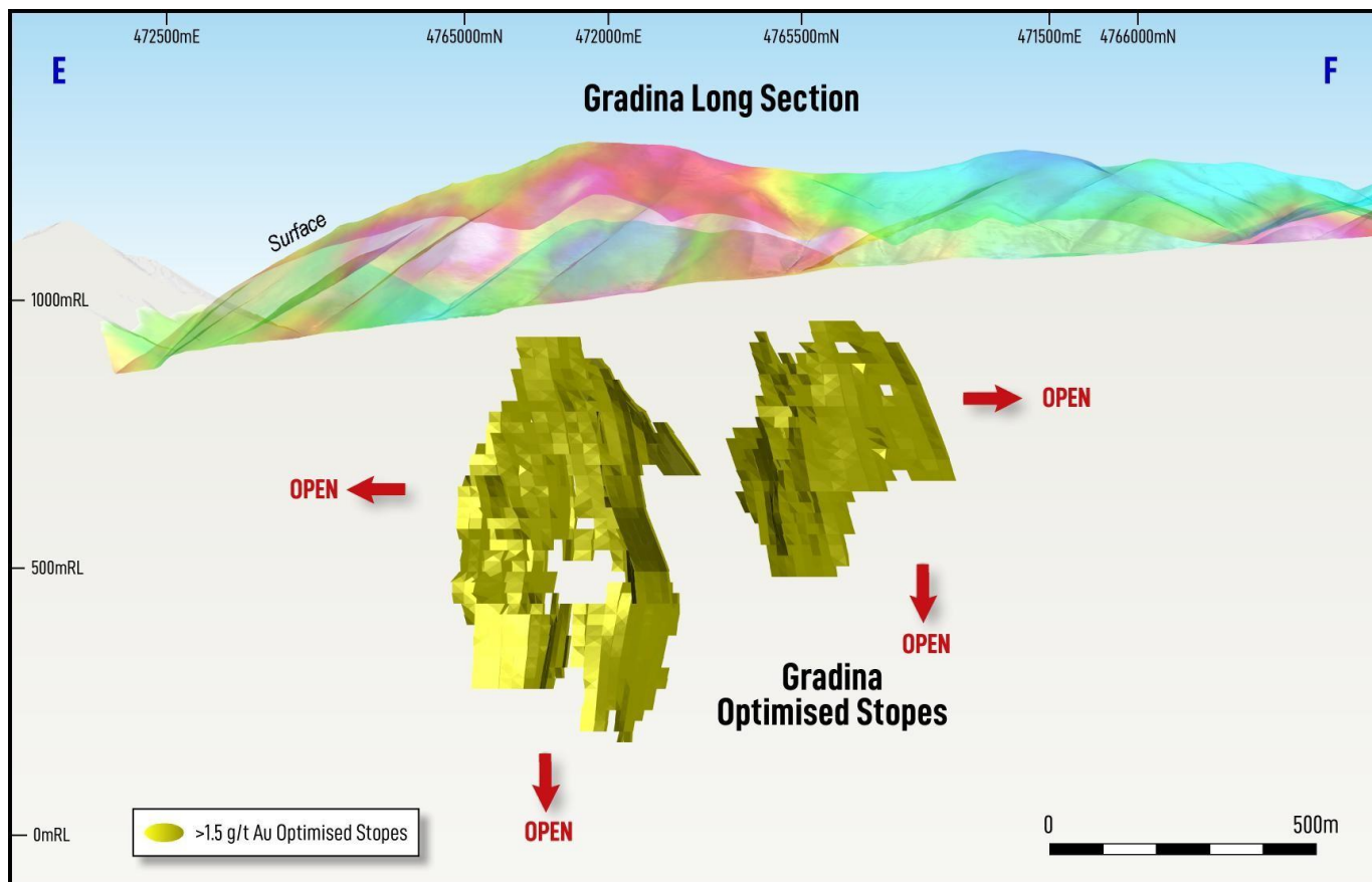
Figure 6. Gradina long section along E – F looking southwest, showing optimised >1.5 g/t Au stopes with gold-arsenic soil geochemical anomalism draped over topography.
