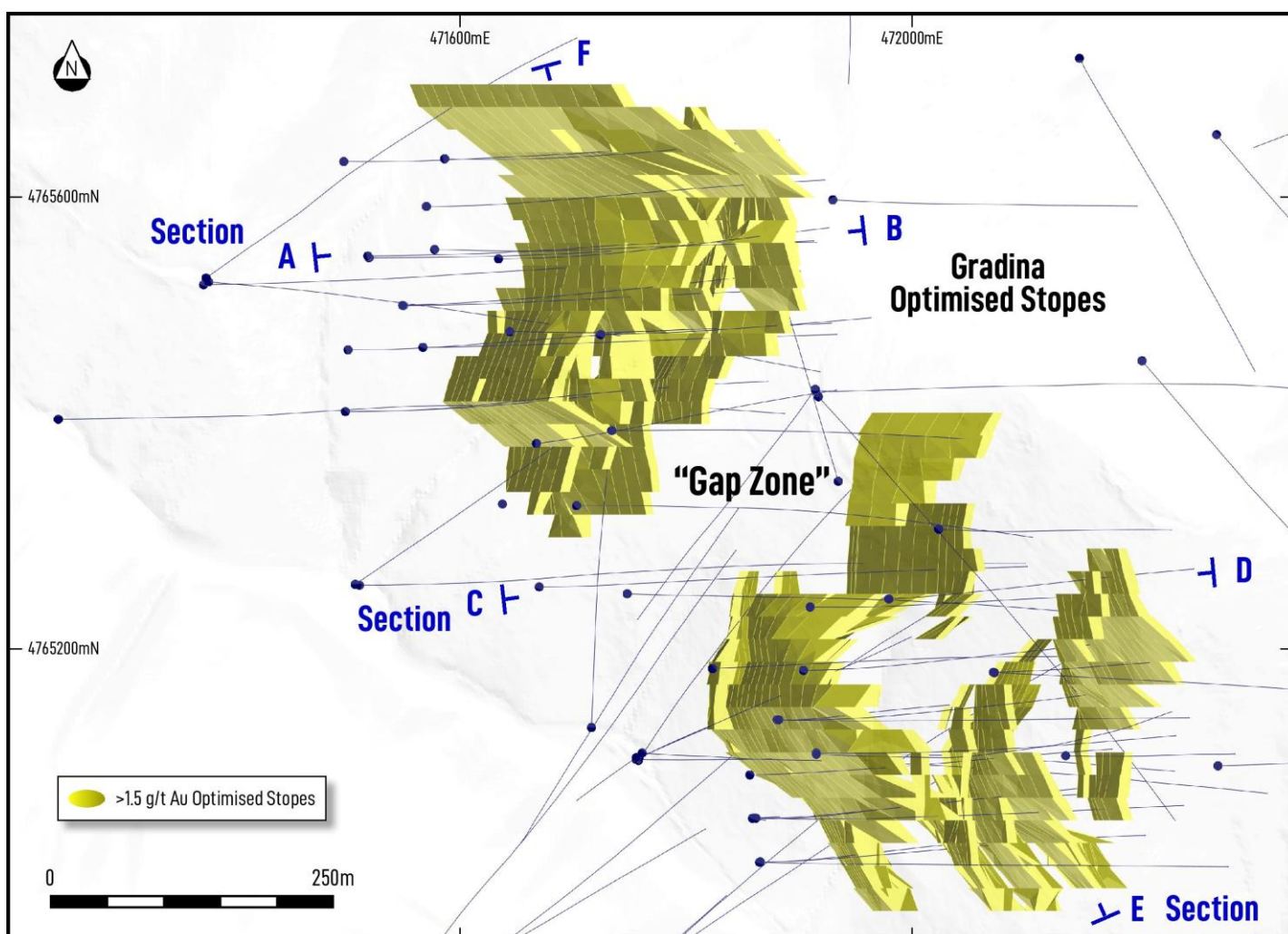
Figure 3. Gradina plan view map showing drill traces and deposit footprint (>1.5g/t Au optimised stopes) with background topography and section labels for subsequent figures.
