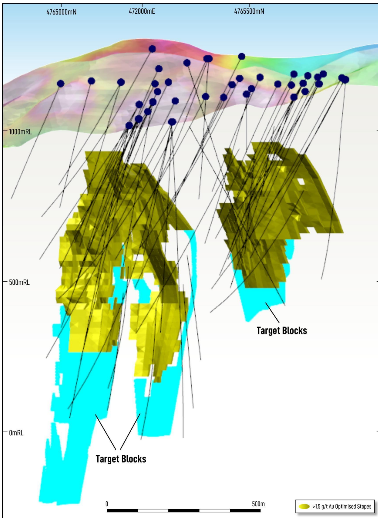
Figure 7. Gradina long section along E – F looking southwest, showing optimised >1.5 g/t stopes constraining Inferred Resources and drillhole traces.
