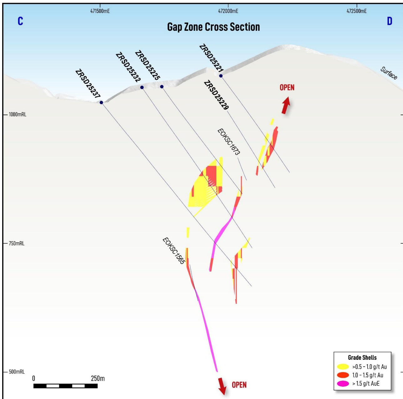
Figure 5. Gradina cross section along E - F, looking north, showing drill traces and >0.5g/t Au model blocks.
