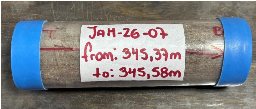
Figure 6. Lexan tube sample for Relative Brine Release Capacity test
