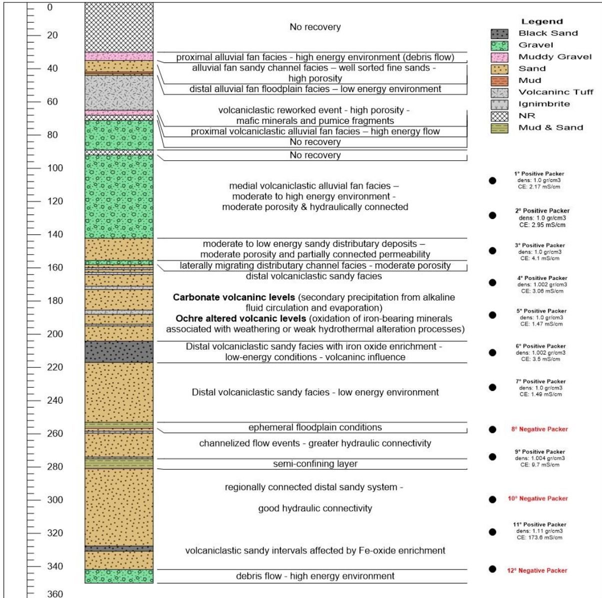
Figure 5. Lithological column from well seven at 350m depth.
