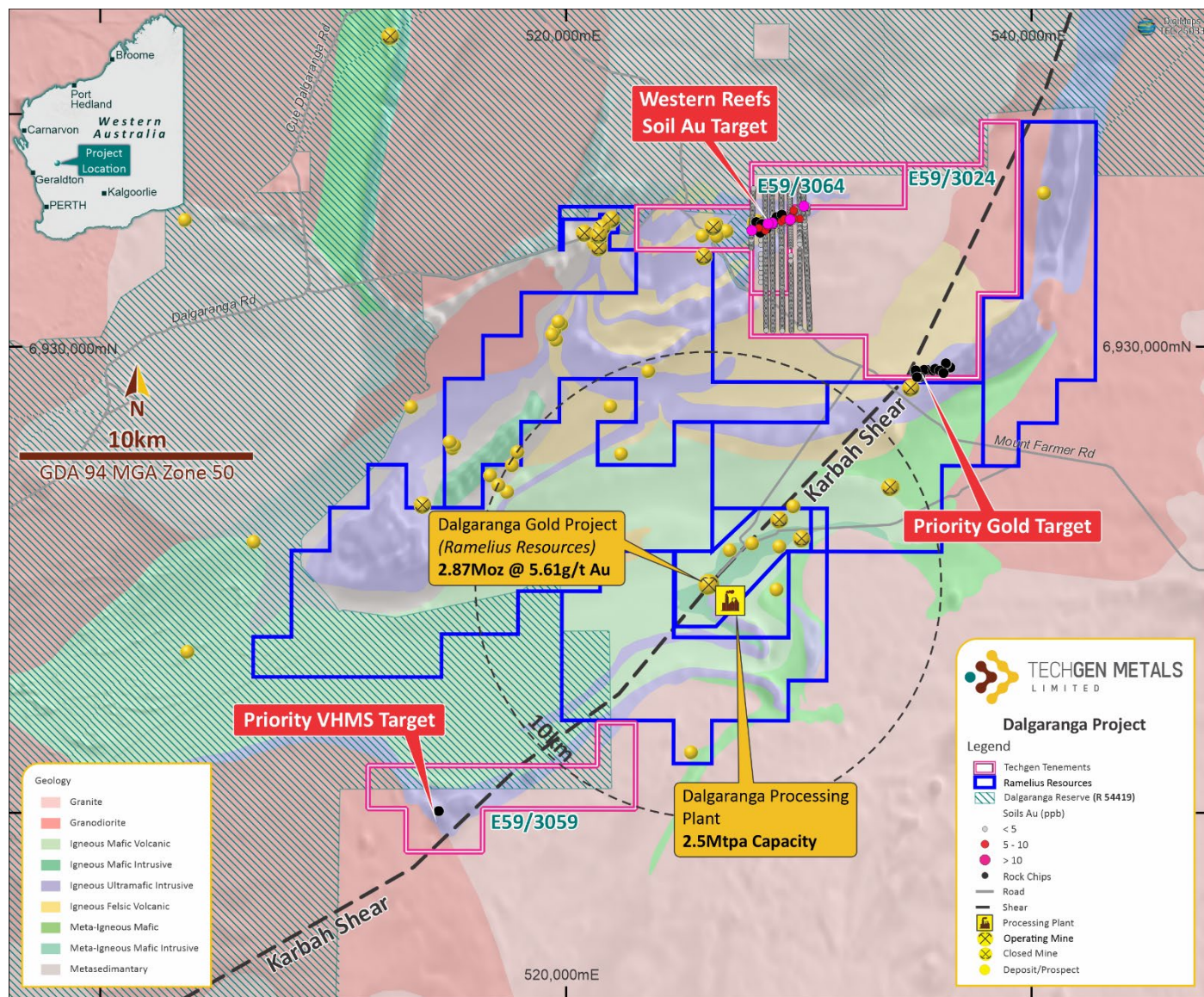
Figure 2: Location of the Western Reefs Au soil target at the Dalgarama Gold Project over geology.
