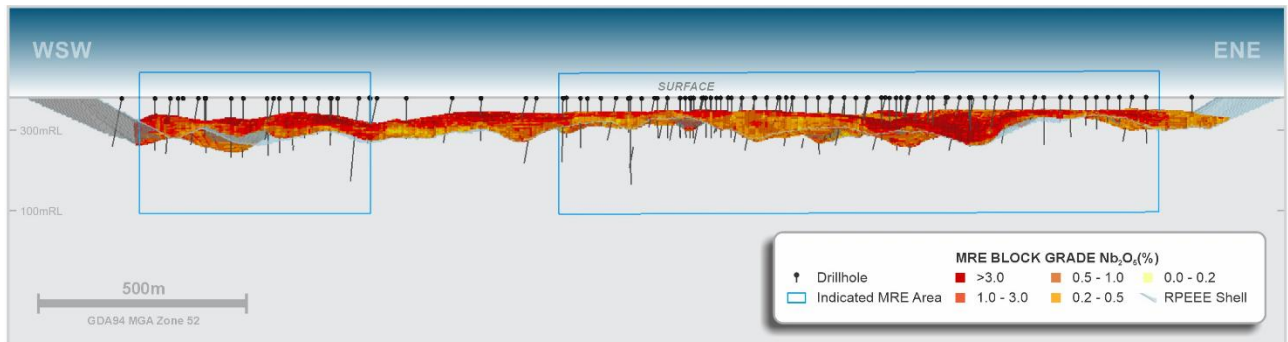
Figure 8: Long section (looking NNW, excl. overlying transported cover)
