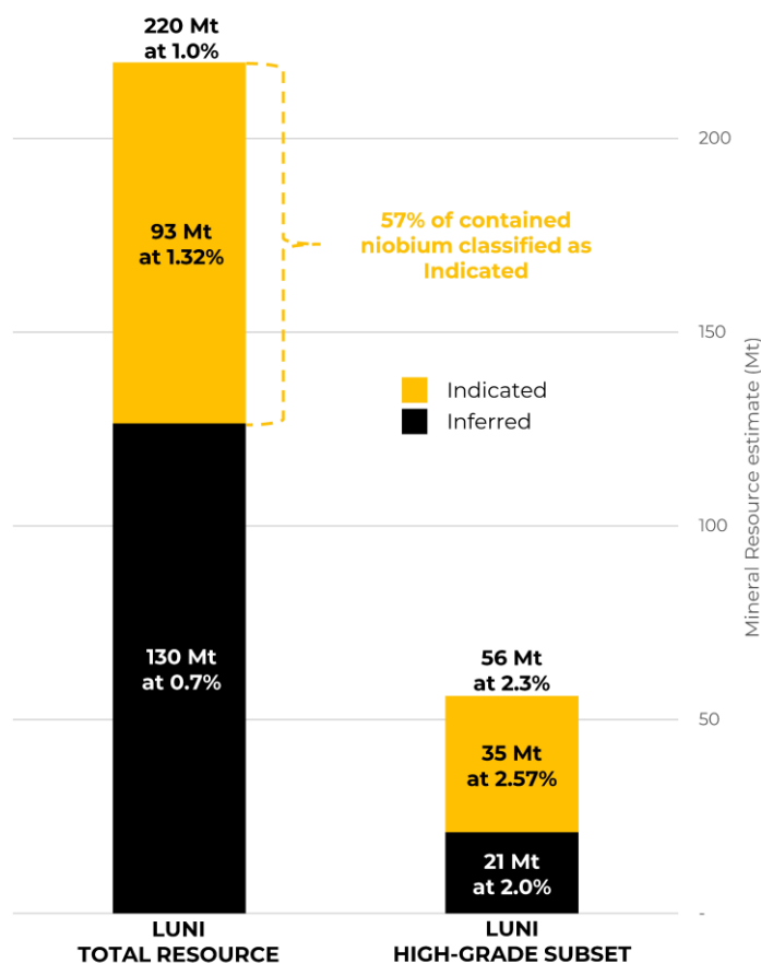
Figure 2: Luni MRE and high-grade subset (Nb 2 O 5 )
