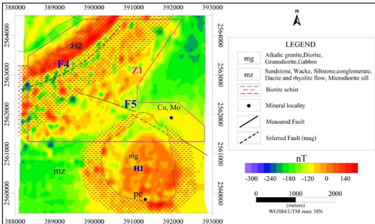
Figure 4. Geological Map, Magnetic Anomalies and Their Inferences of the Z1 Area
