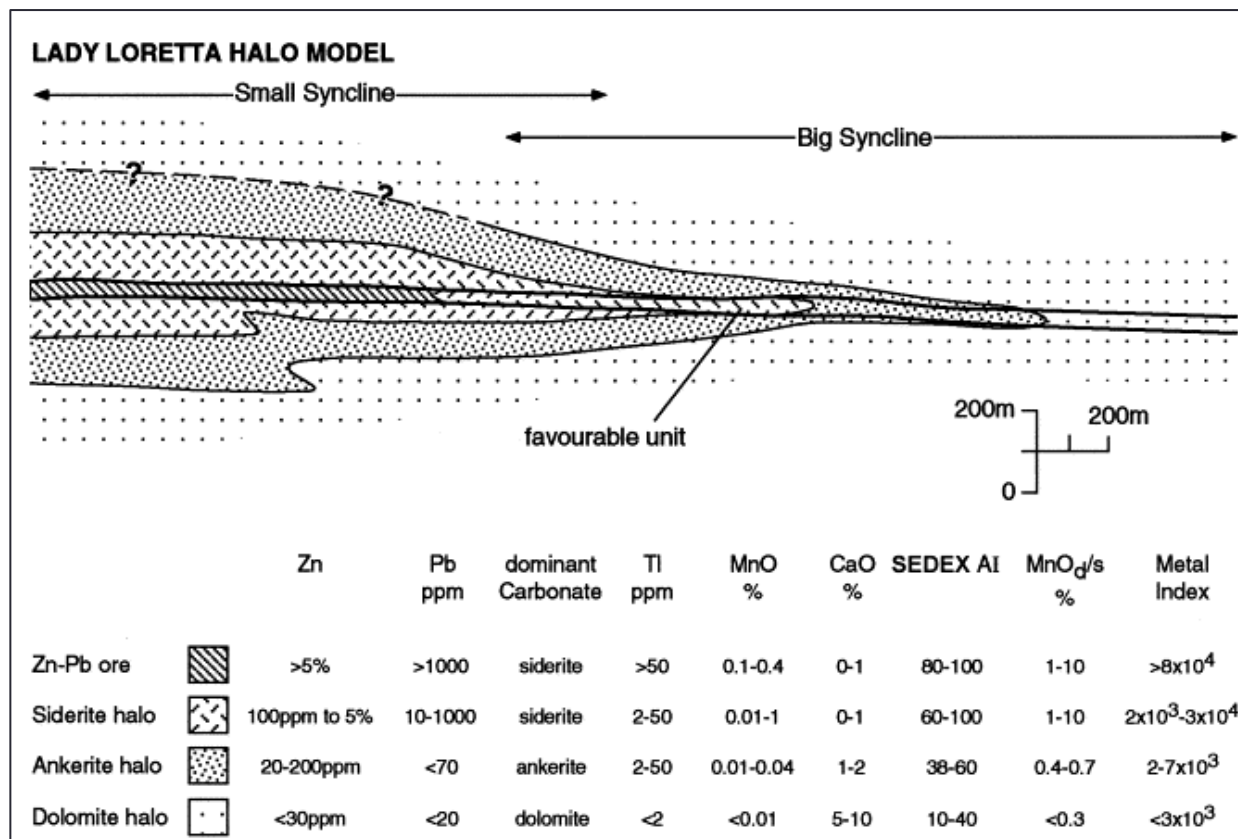
Figure 3. Alteration halo model (pre-folding) for the Lady Loretta Deposit (Large and McGoldrick, 1998).
