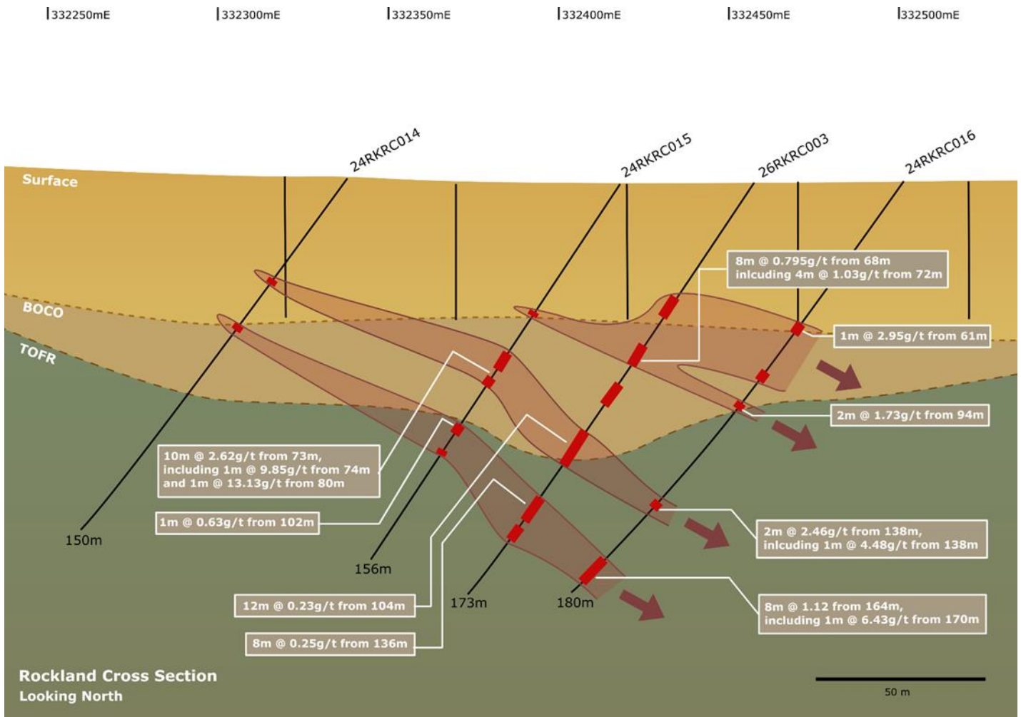
Figure 2: Interpretive cross section of drill line 6639220N
