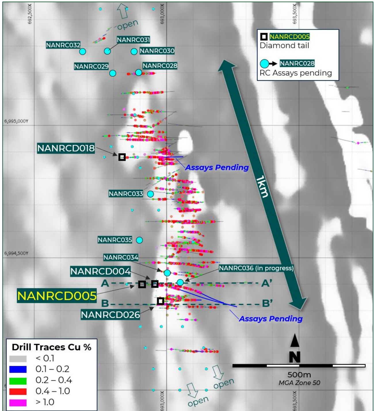
Figure 1. Nanadie Deposit aeromagnetic imagery and downhole copper values in all previous drilling 2,3 projected to surface, showing the location of completed diamond tails and NANRCD004 and NANRCD005 (labelled), planned Phase 2 RC drill collars (small blue dots), and completed RC holes (labelled).
