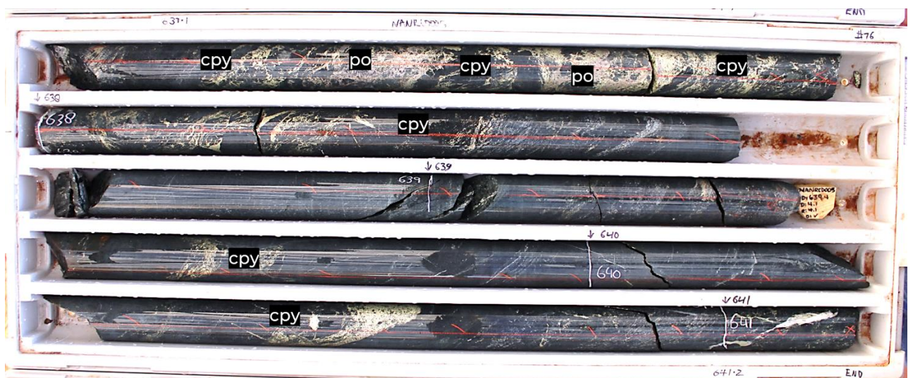
NANRCD005 637.1.8-641.2m - part of 25.3m zone averaging 2.5% logged chalcopyrite
