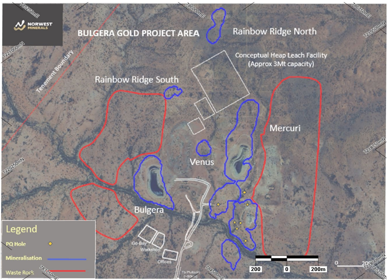
Figure 1 – Preliminary Bulgera heap leach design showing PQ core locations, conceptual heap leach infrastructure, areas of surface gold mineralisation, and proposed waste storage areas.
