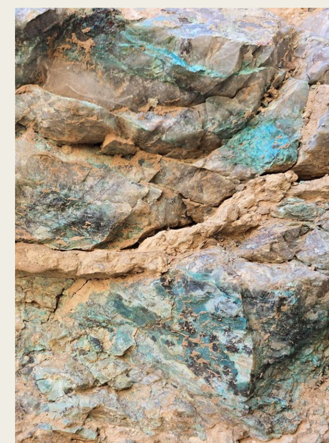
Examples of widespread copper mineralisation at Donkey Hill prospect at Chalkos
