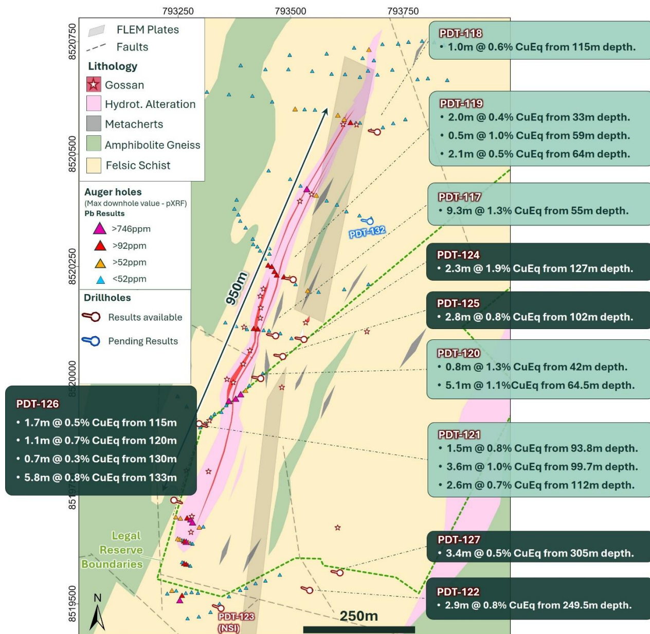
Figure 2: Touro Prospect plan map including drilling to date, gossans and the hydrothermal alteration zone. The FLEM Plates are included in shaded grey.
