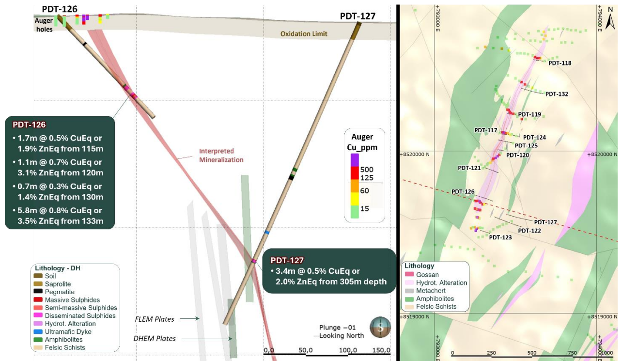
Figure 4: Cross section through holes PDT-126 and PDT-127.
