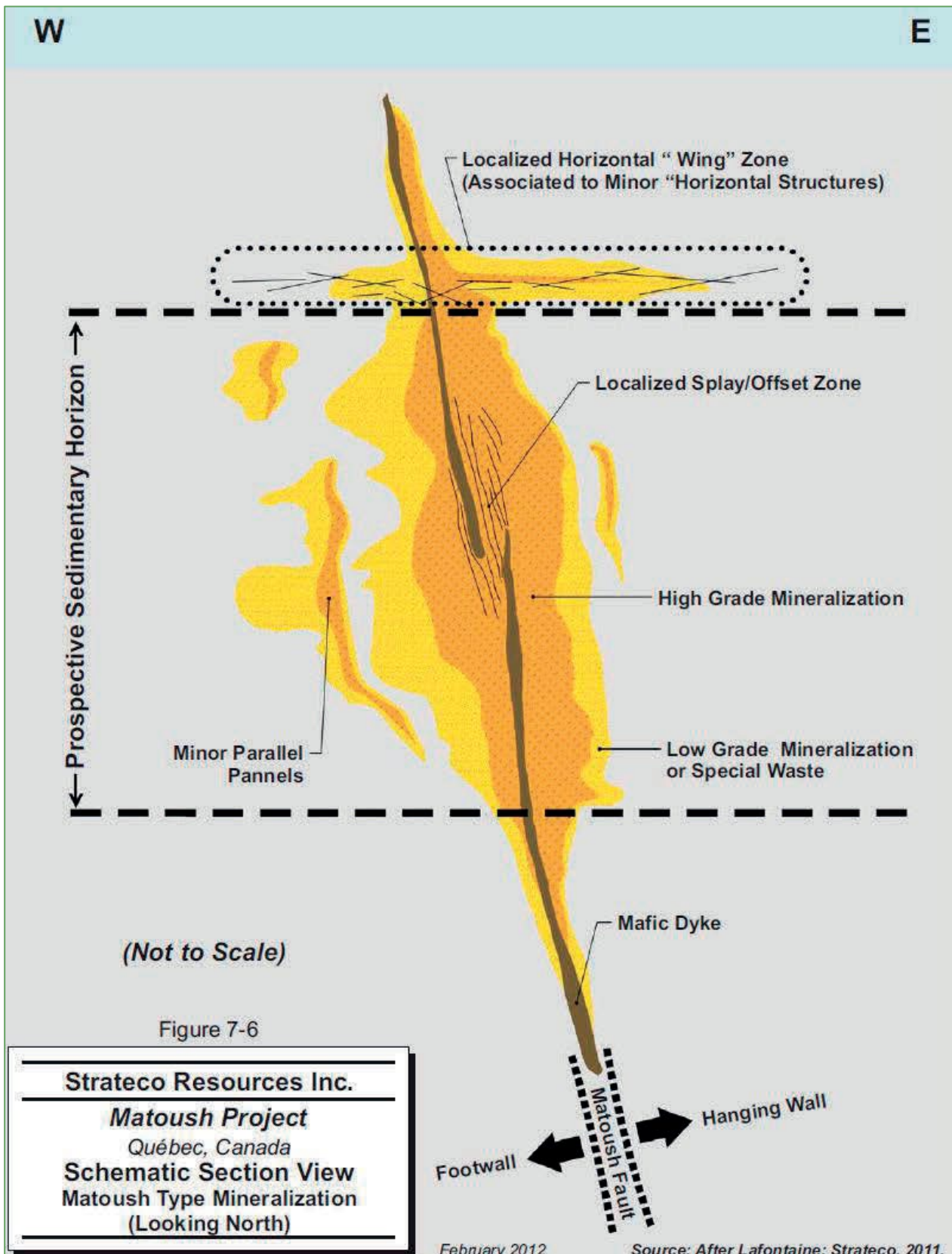
Figure 23: Schematic section of Matoush mineralisation envelope (looking North) Source: RPA, 2012
