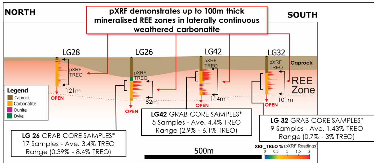
Figure 4: N–S cross-section showing selected historical drill holes sampled as part of due diligence. Histograms represent detectable downhole portable XRF (pXRF) responses for combined REE oxides ( \text{CeO}_2 + \text{La}_2\text{O}_3 + \text{Nd}_2\text{O}_3 + \text{Pr}_6\text{O}_{11} ), displayed on a logarithmic scale. Locations and average laboratory assay results for downhole grab samples taken from historical drill core during due diligence are also displayed.
