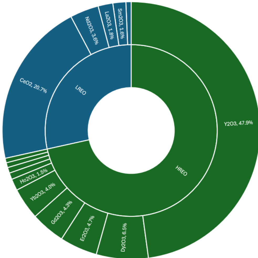
Figure 2: Rare Earth Oxide basket composition of the +300 -1mm SG -3.5+3.0 stream generated using HLS
