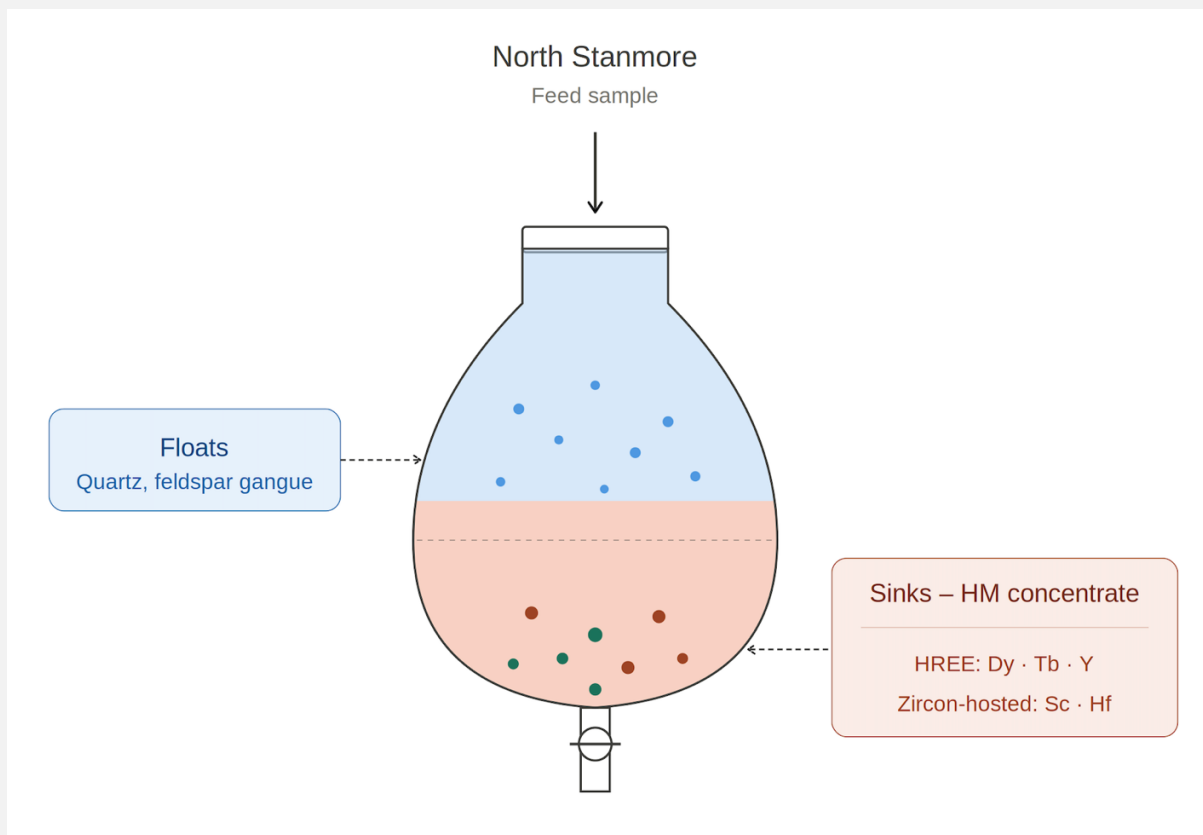
Figure 1: Typical Schematic of Heavy Liquid Separation (HLS) conducted on North Stanmore feed sample. Not to scale.
