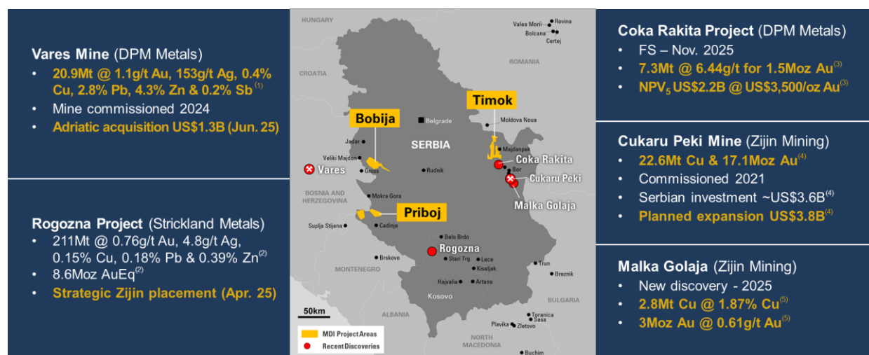
Figure 10: Location of Middle Island projects within world class mineral province.
