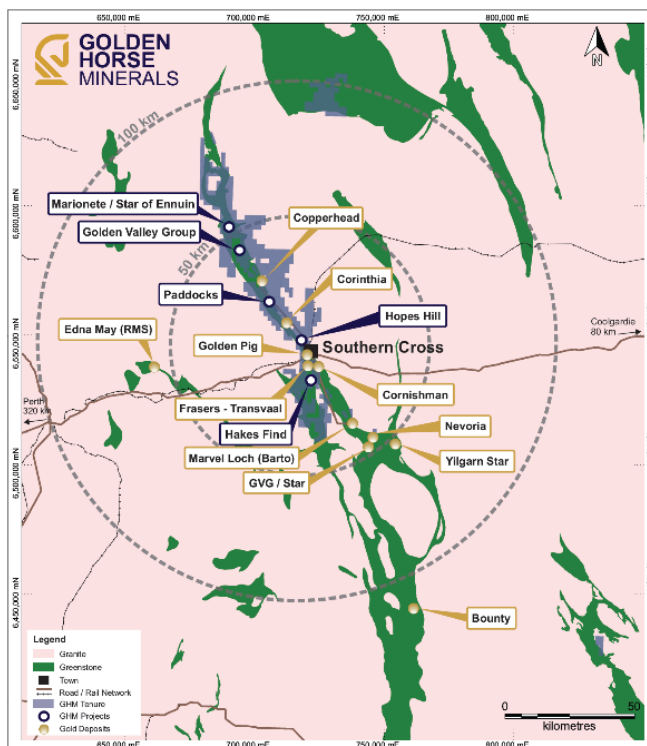
Figure 15: GHM regional prospects
