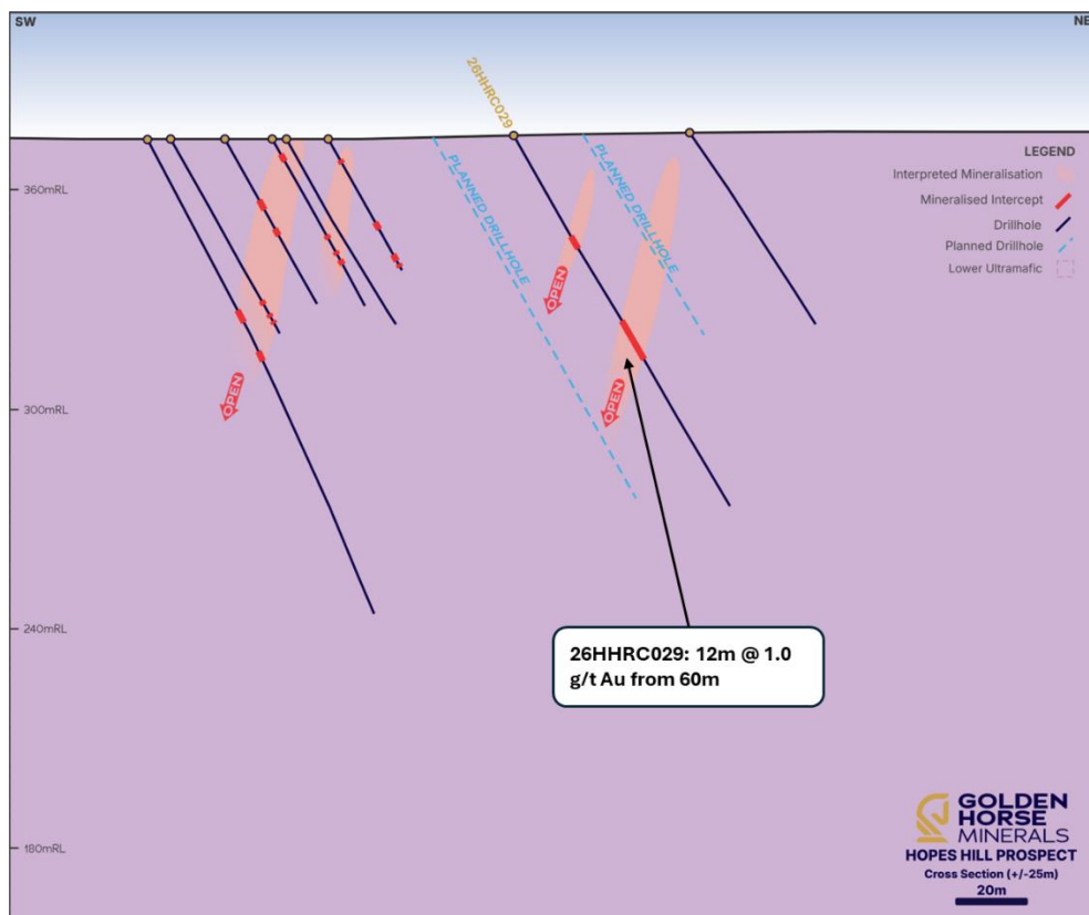
Figure 11: Cross Section of Hopes Hill North showing 26HHRC029 (12m @ 1.0 g/t Au).
