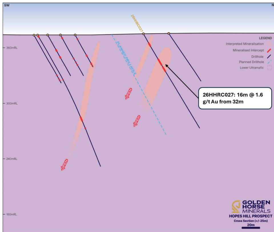
Figure 8: Cross Section of Hopes Hill North with 26HHRC027 (16m @ 1.6 g/t Au).
