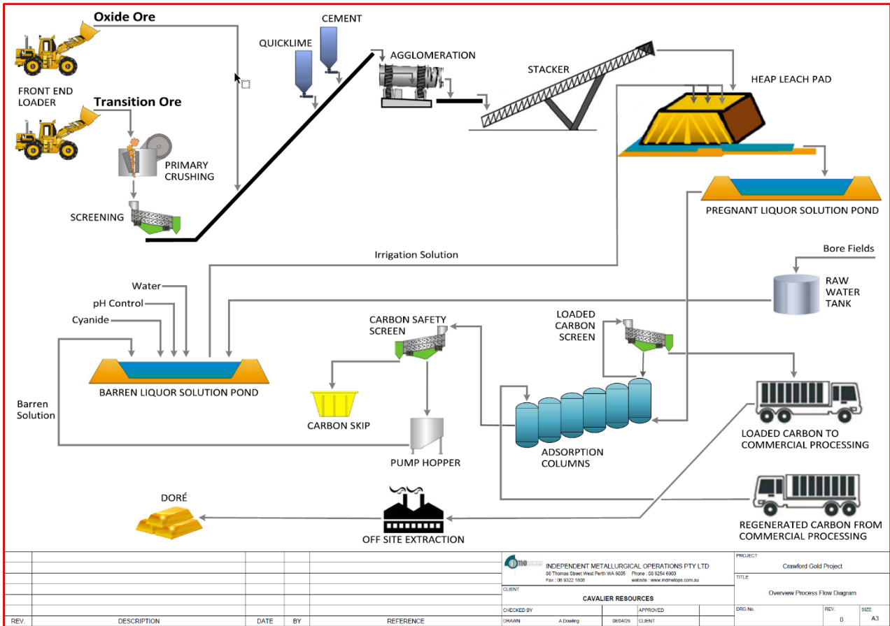
Figure 2: Updated Process Flowsheet
