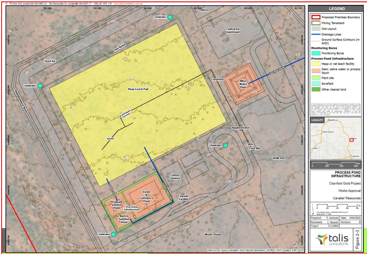
Figure 3: Process Area, Detailed Layout
