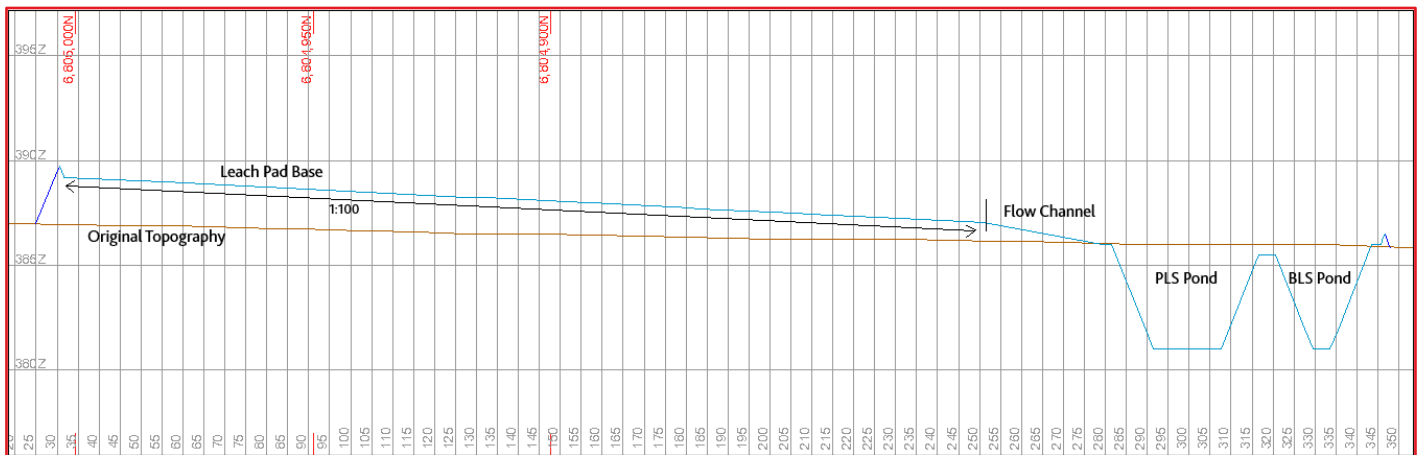
Figure 5: Heap Leach Pad and Pond Section
