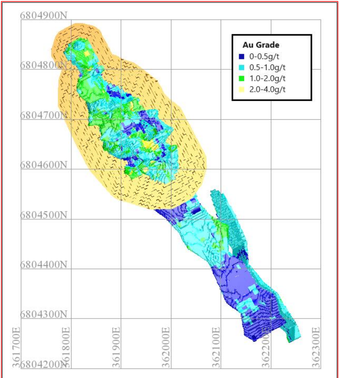
Figure 7: Selected Crawford Oxidised Material Whittle Optimisation Shell (with Domained Resources)
