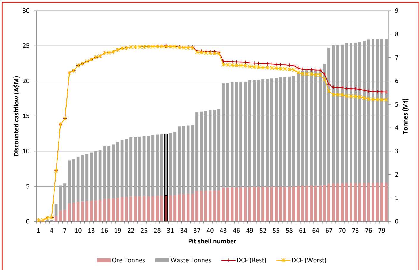
Figure 6: Crawford Oxidised Material Base Case Pit by Pit Graph
