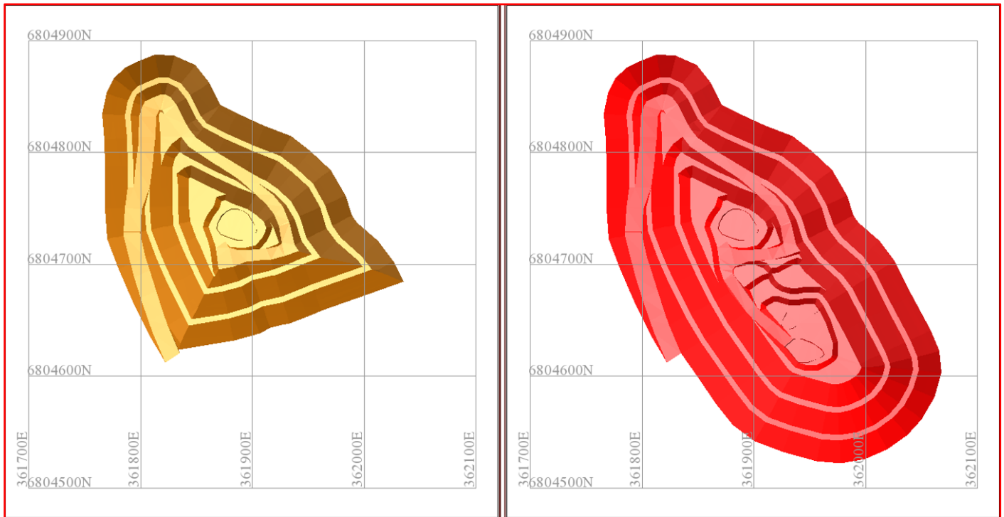
Figure 8: Crawford Oxidised Material Pit Design Stages 1A (left) and 1B (right), Plan View
