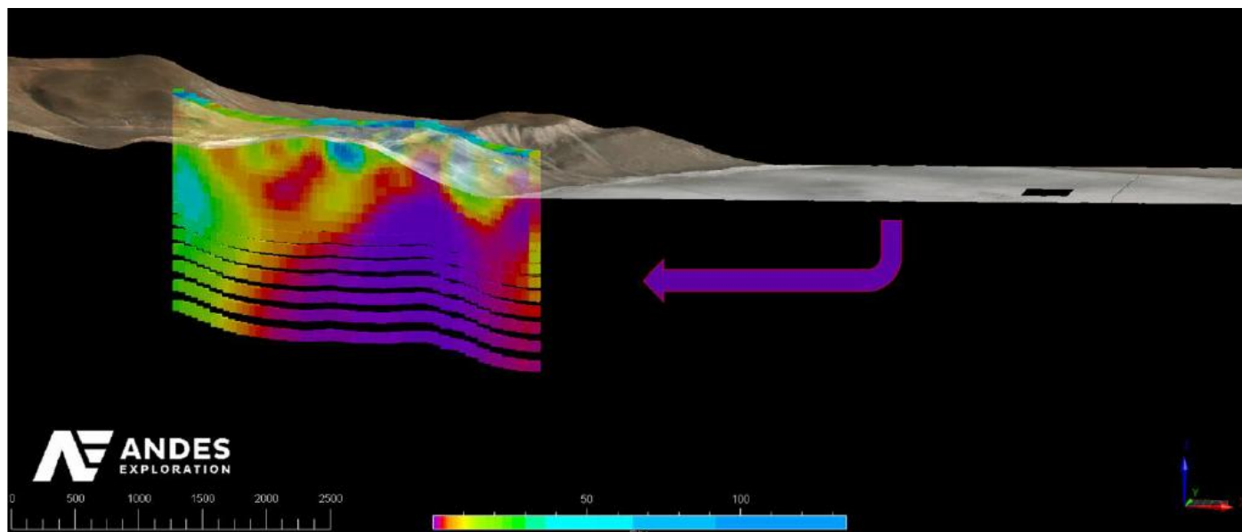
Figure 3 – Cross Section (L1500) Highlighting Depth-Continuous Conductive Zone Interpreted as a Brine Target
