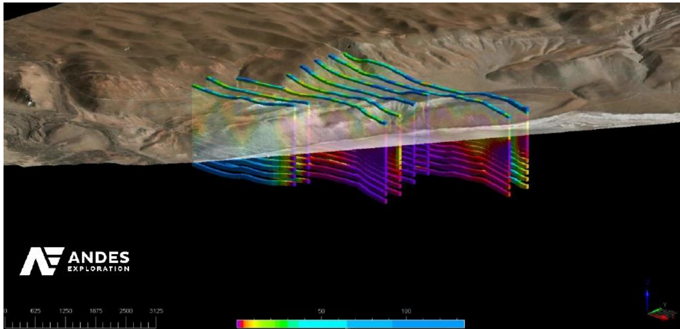
Figure 1 – 3D CSAMT Model Highlighting Continuous Conductive Zones at Depth Across Mito
