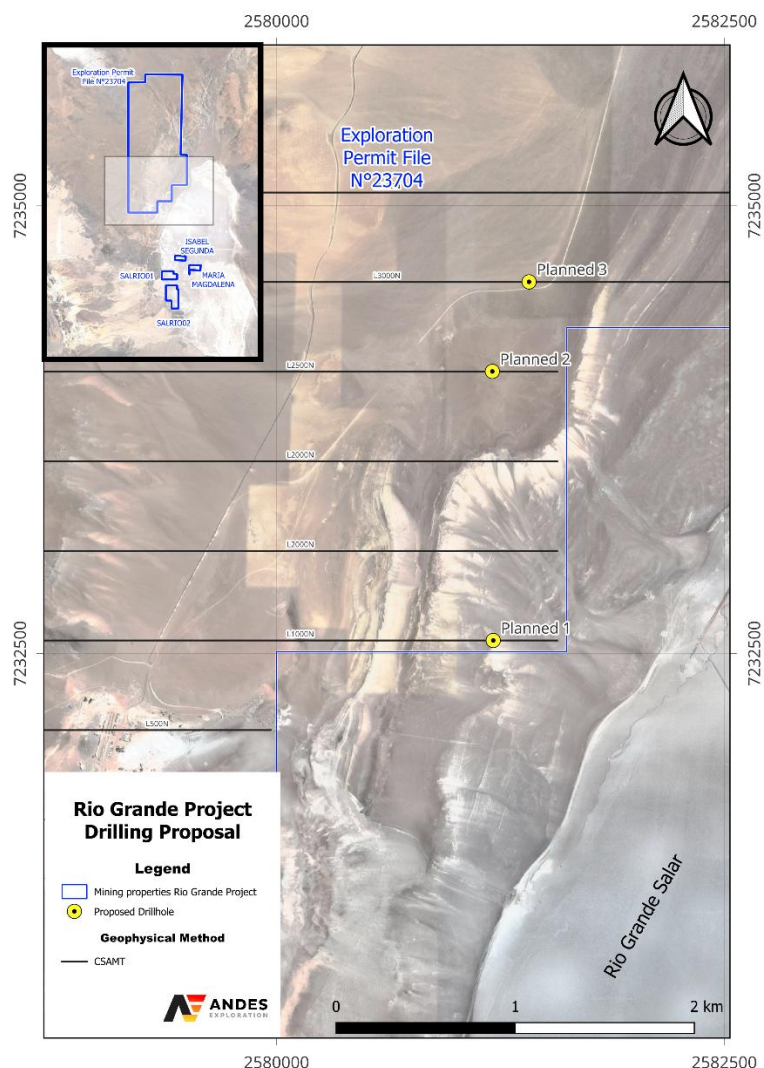
Figure 6 – Proposed Drillhole Locations for High-Confidence Brine Targets at Mito
