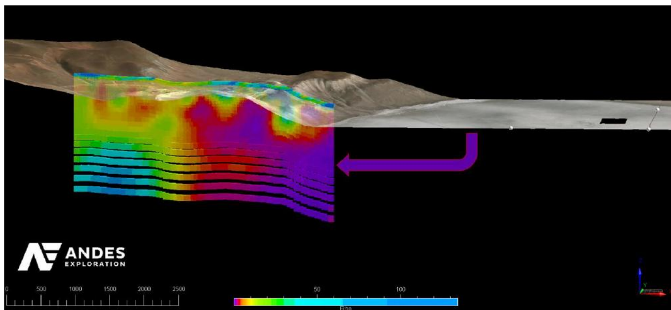
Figure 2 – Cross Section (L1000) Highlighting Depth-Continuous Conductive Zone Interpreted as a Brine Target
