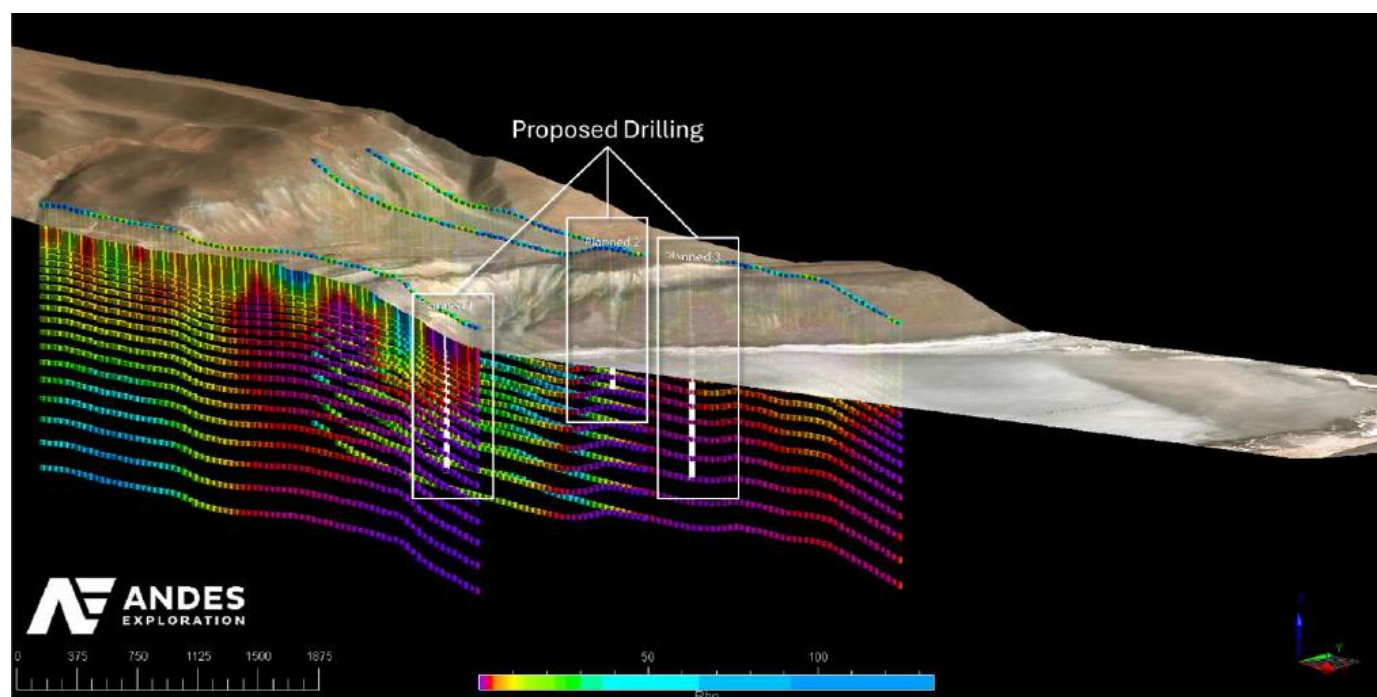
Figure 5 – Planned Drilling Targeting Large-Scale Conductive System to Support Resource Expansion at Mito
