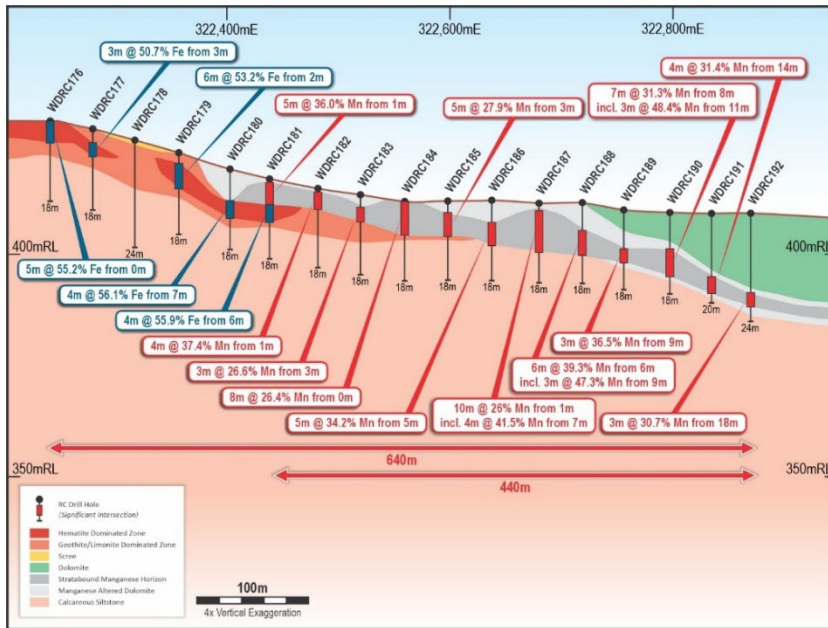
Figure 4. Most northern cross section 7,526,500mN looking to the north showing the location of RC drill holes with shallow high-grade iron and manganese mineralisation. Iron and manganese mineralisation remains open to the north 2 . Cross-section location presented in Figure 2.
