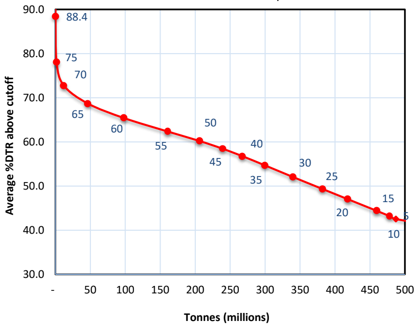
Figure 4 Total Resources Grade Tonnage Curve December 2025
