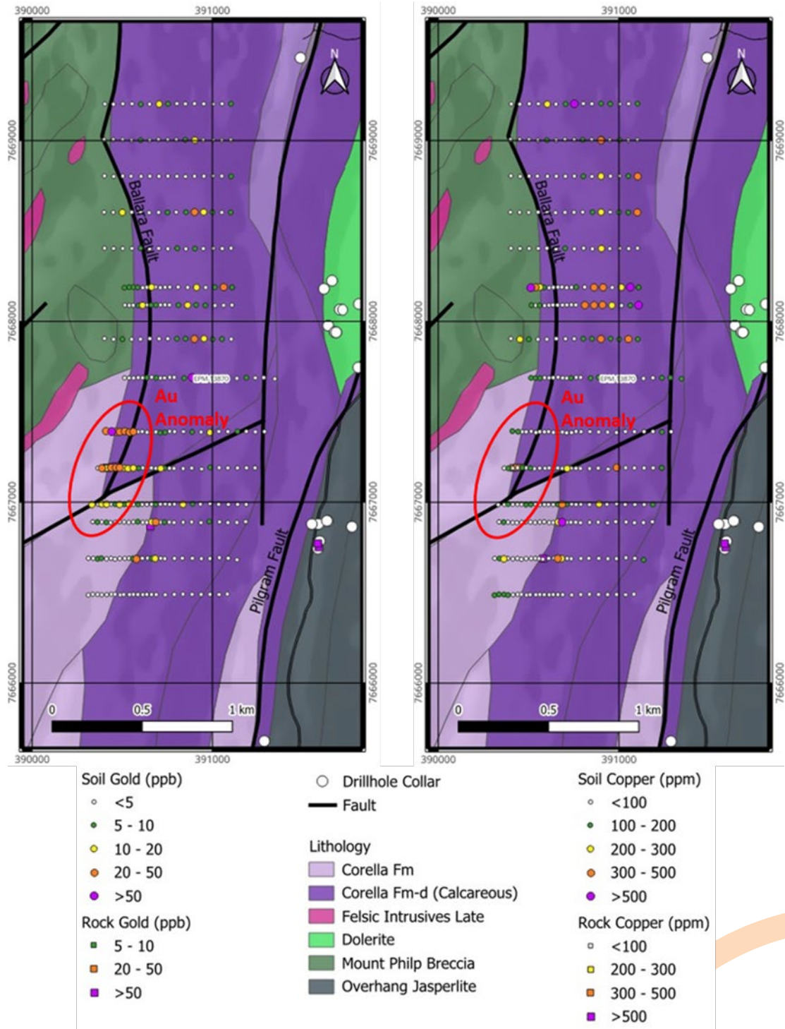
Figure 7. Gold vs copper anomalism in soil and rock chips in the Keyser area. Copper values are from PXRF analysis and Au values are from fire assay. PGN interpreted Geology layer underlain by TMI RTP magnetics with shading from the east. The reader is referred to Table 1 JORC (Balanced reporting) for a discussion on soil sampling.
