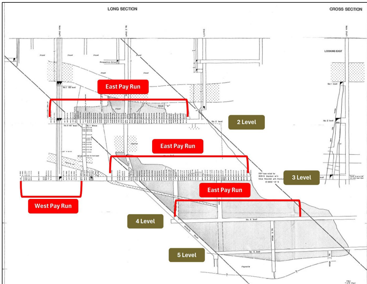
Figure 2: Princess Royal historical gold pay runs calculated from 1982 AMC reports (5 level data missing from this image) Level data is compiled within the appendices.
