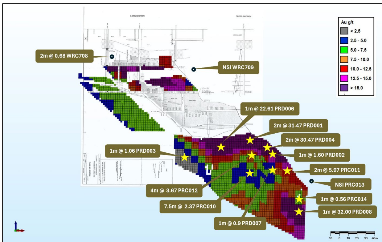
Figure 1: Princess Royal long section looking northwest. Historic mine survey with Exploration Target model and drillhole intercepts (metres @ grams per tonne, drillhole ID)
