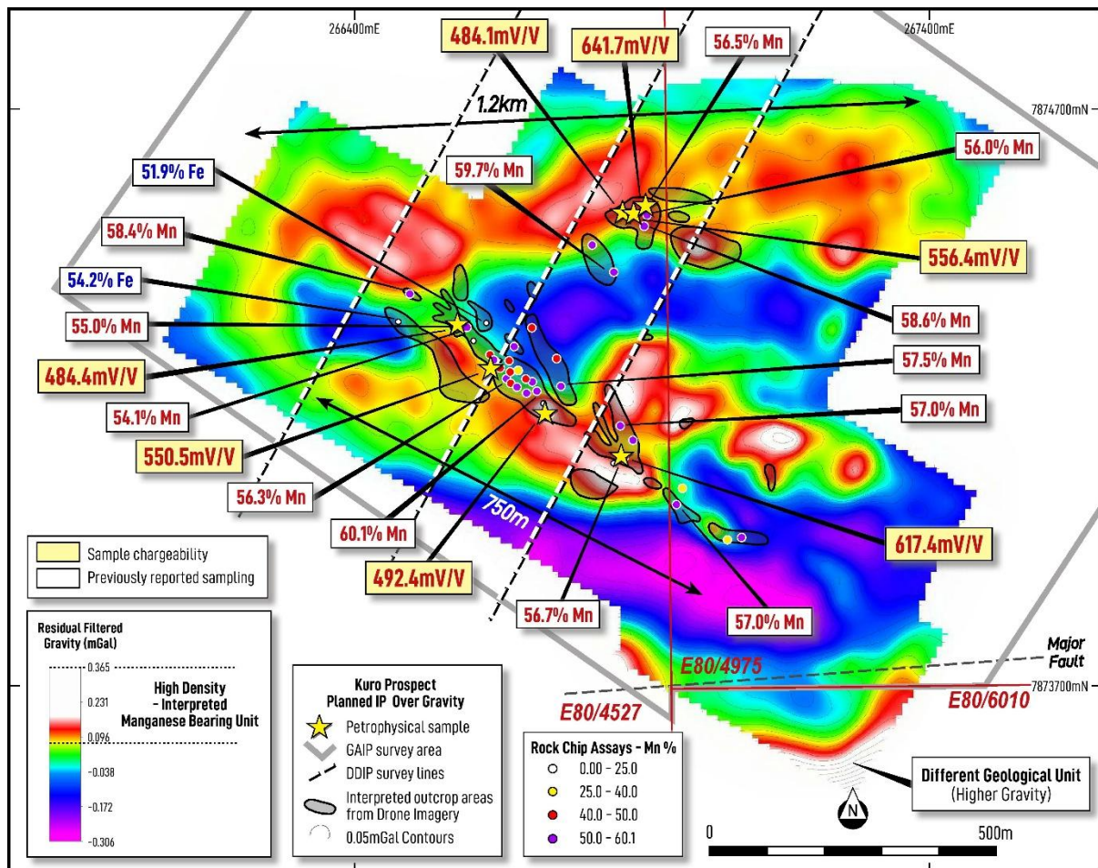
Figure 1. Petrophysical sample locations, highlighting high chargeability results across the Kuro Prospect area, showing planned GAIP survey area and example DDIP lines. Background coloured imagery is ground gravity data (with hot colours indicating dense material – interpreted to represent manganese mineralisation), black polygons are interpreted manganese outcrop, and dots with Mn% callouts are rock chip sample locations.
