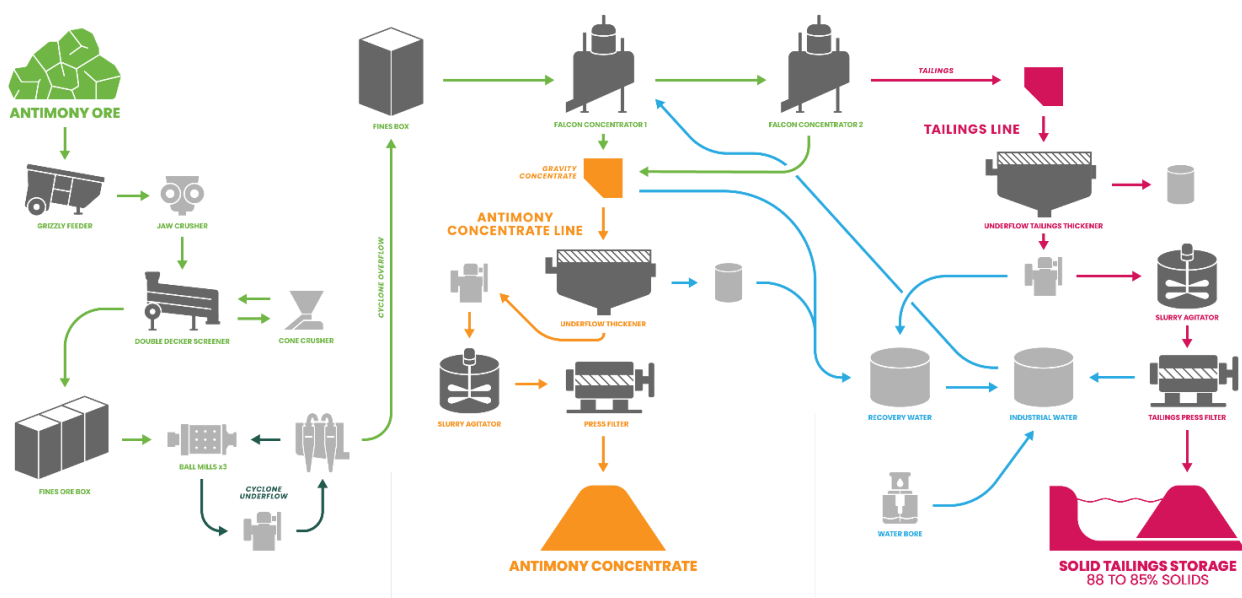
Figure 3: Tecamatlán Plant Proposed Gravity Circuit Flowsheet
